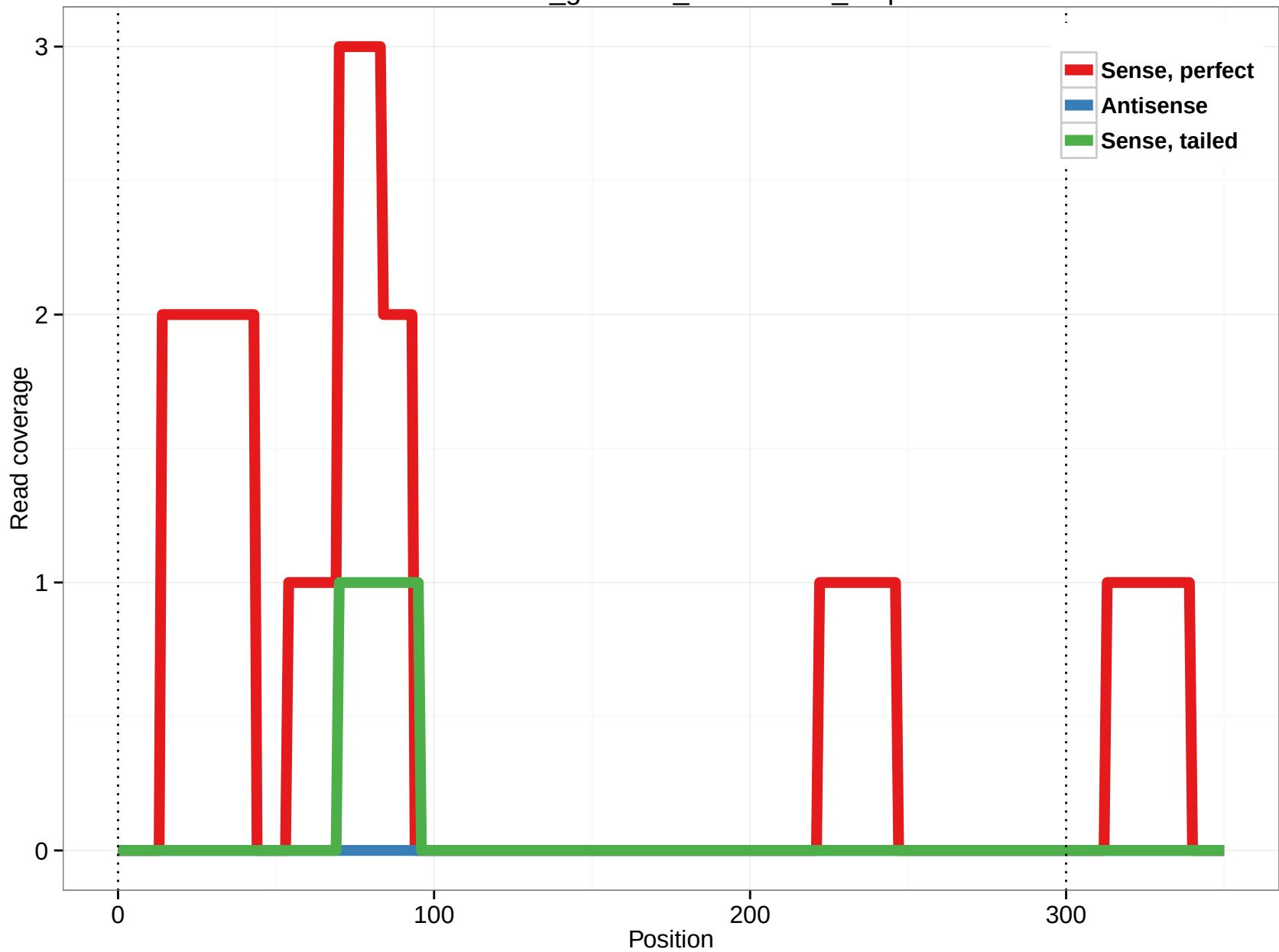
rheMac3_genscan_chr11.1774_4.3p
