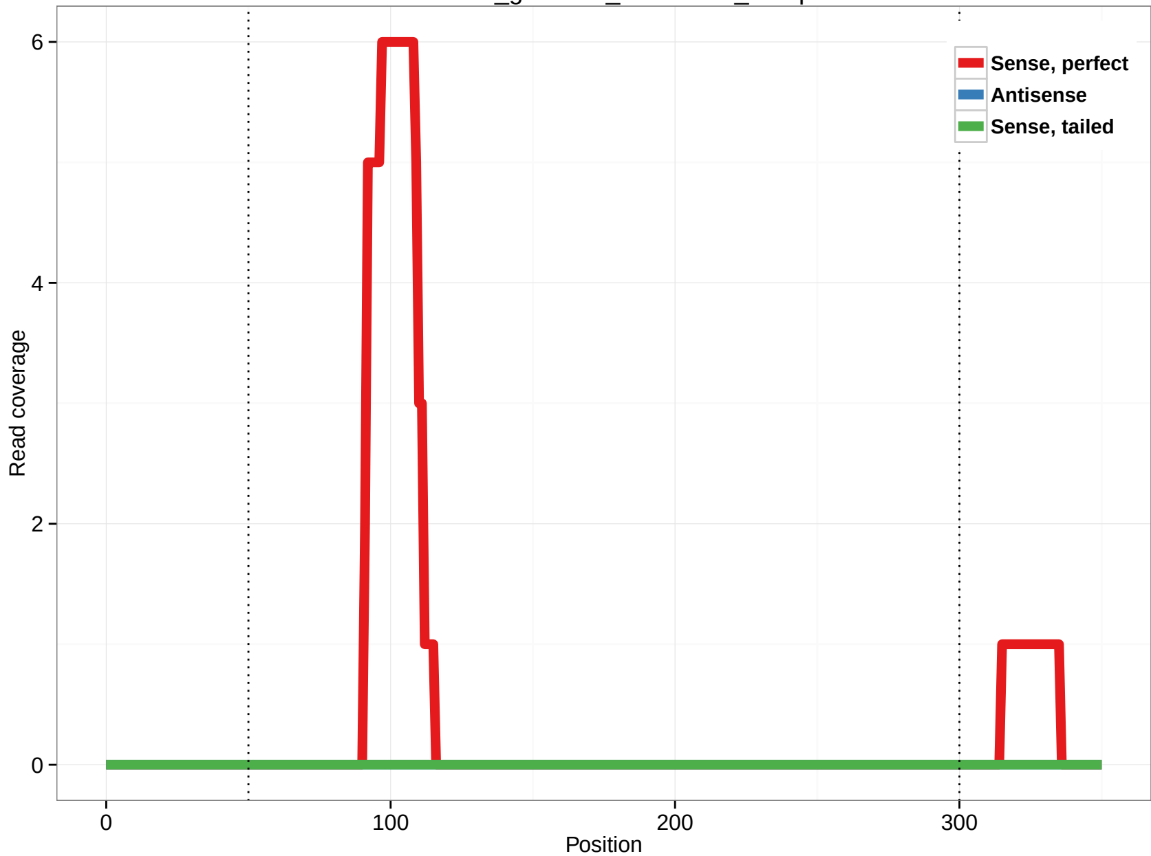
rheMac3_genscan_chr11.171_26.3p
