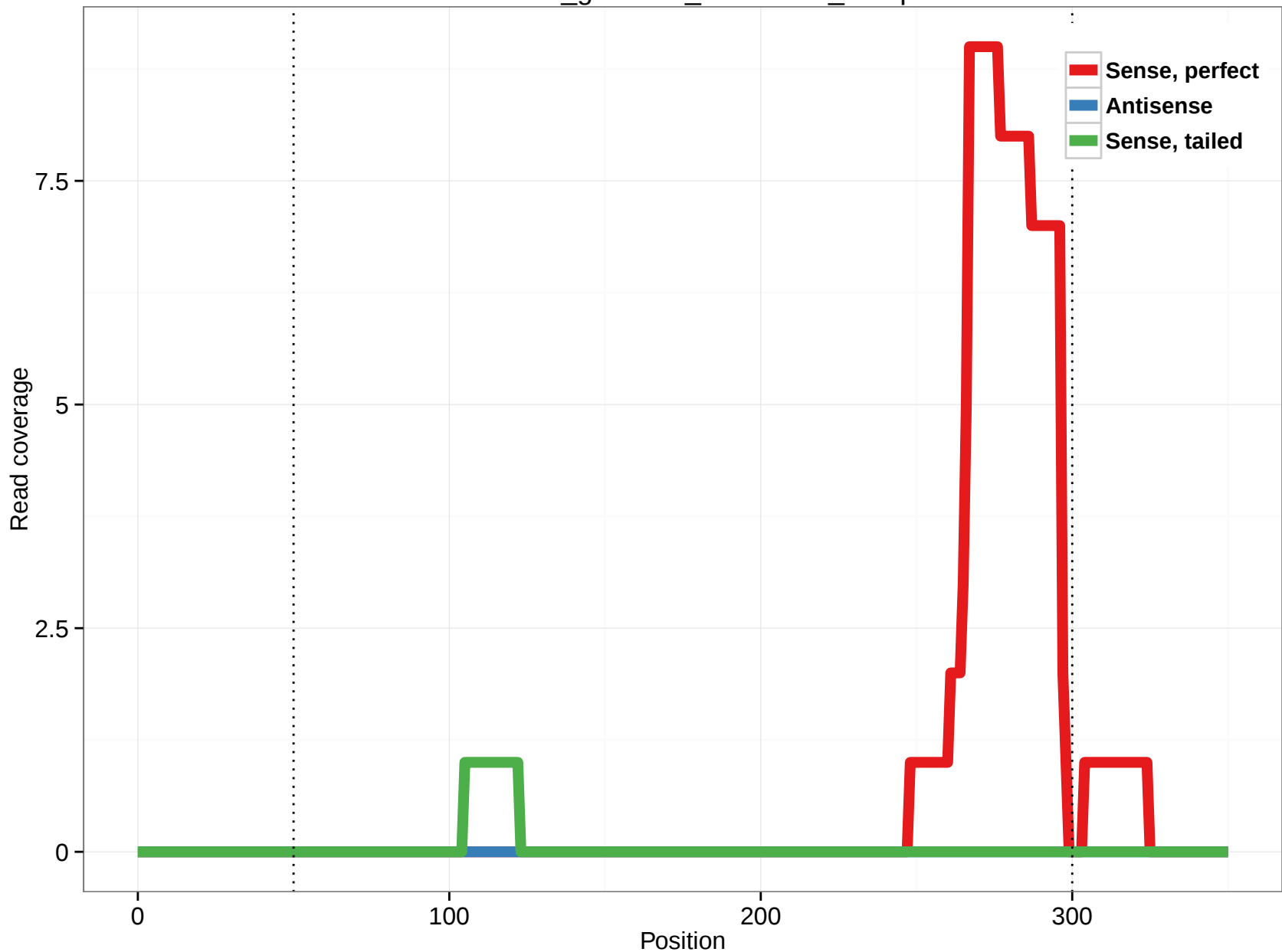
rheMac3_genscan_chr11.171_22.5p
