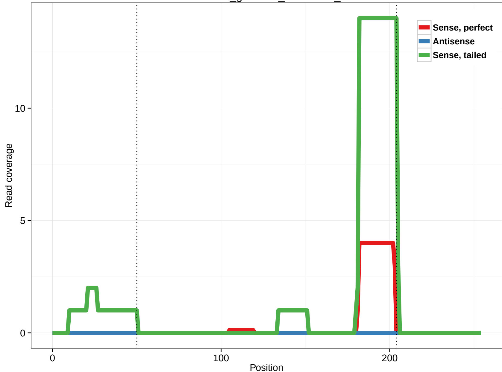
rheMac3_genscan_chr11.168_3
