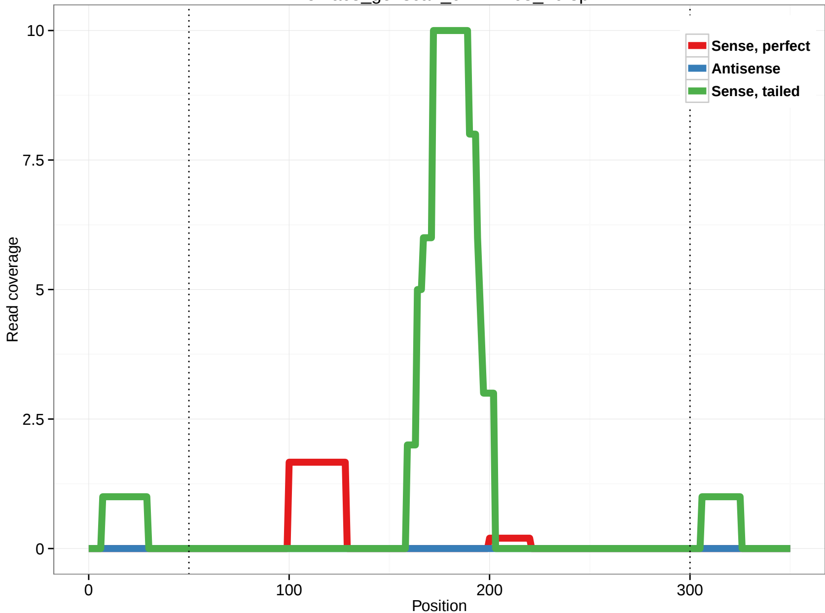
rheMac3_genscan_chr11.168_16.3p
