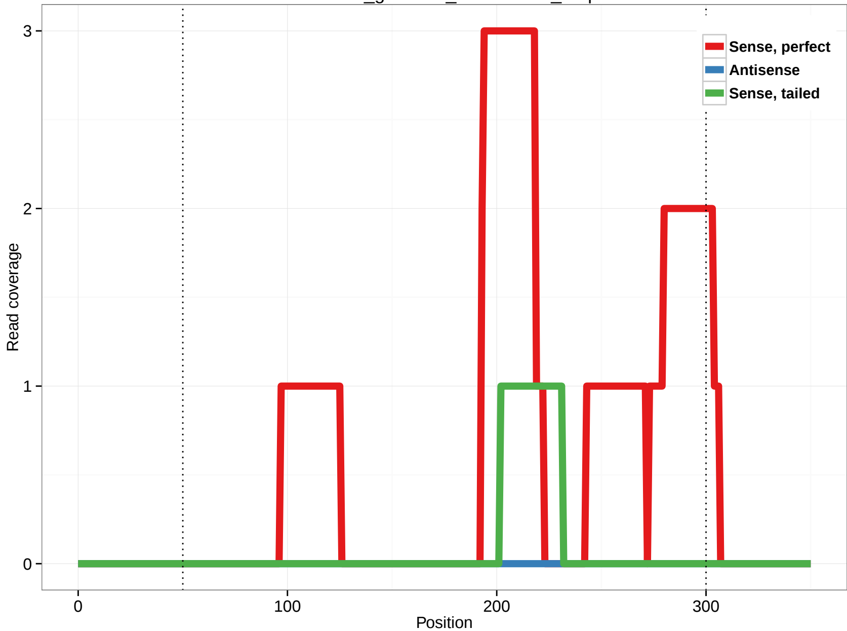
rheMac3_genscan_chr11.1647_2.3p
