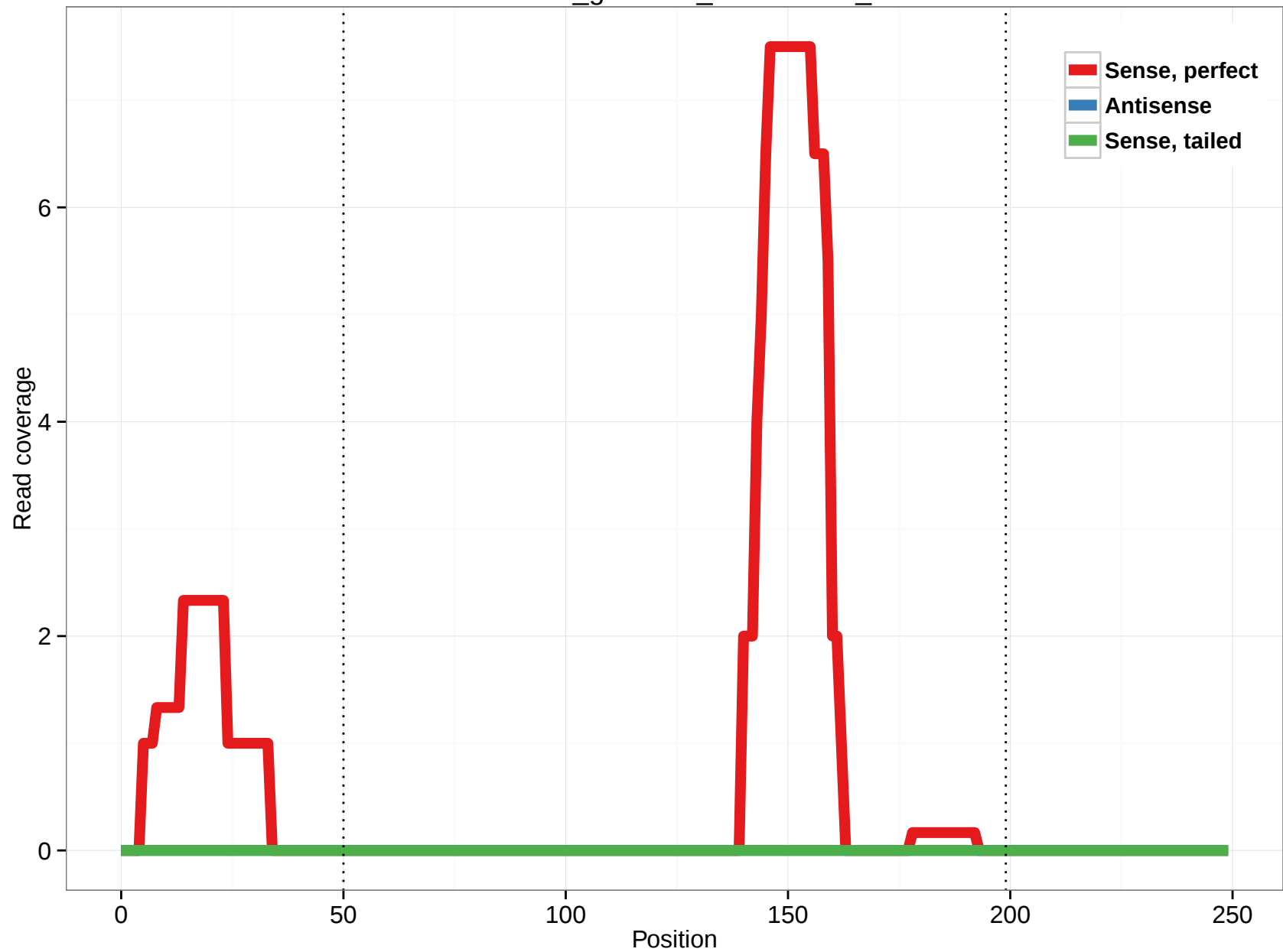
rheMac3_genscan_chr11.1639_1
