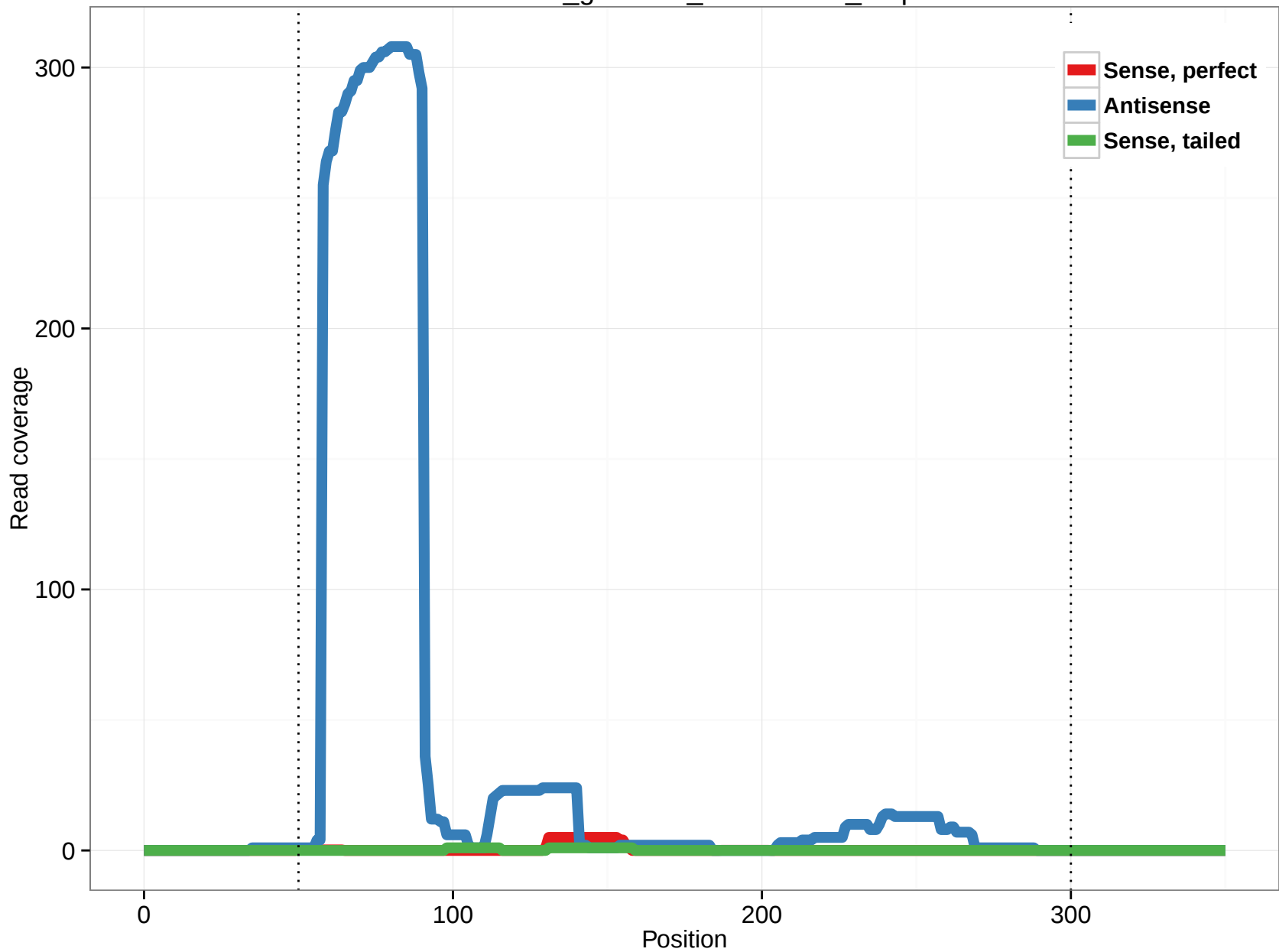
rheMac3_genscan_chr11.1602_4.5p
