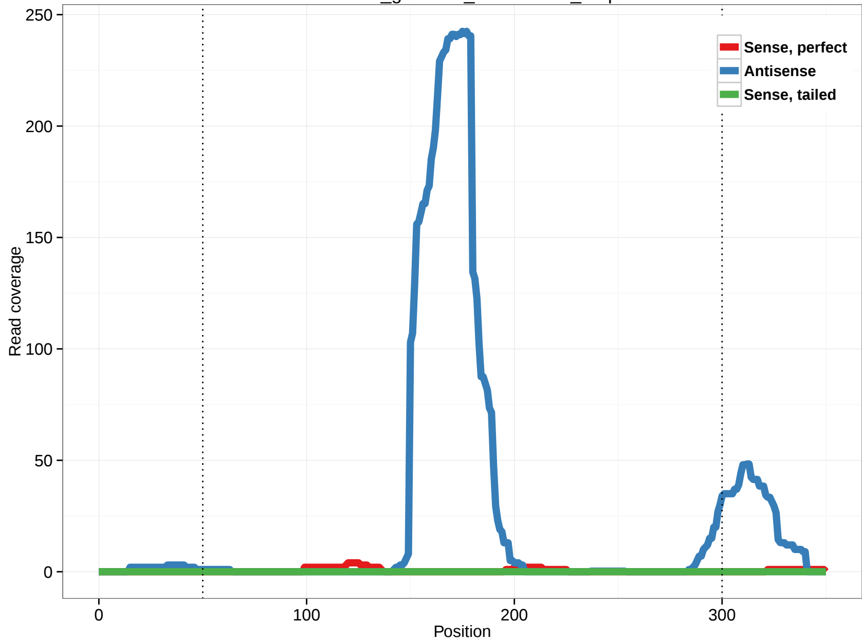
rheMac3_genscan_chr11.1602_3.3p
