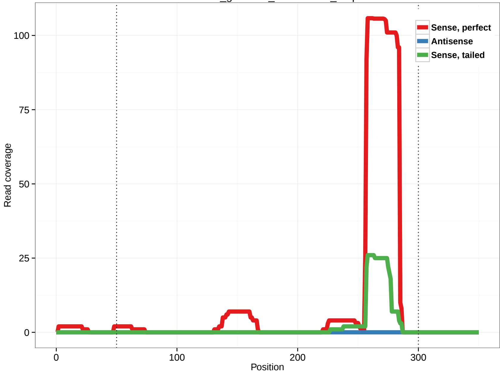
rheMac3_genscan_chr11.1598_3.3p
