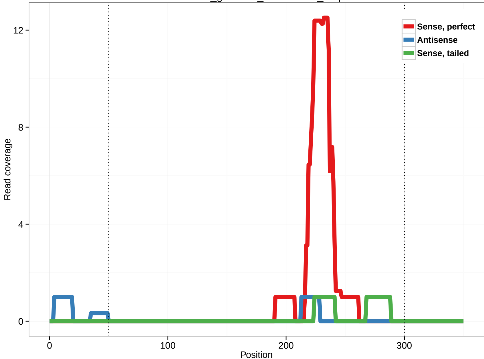
rheMac3_genscan_chr11.1594_7.5p
