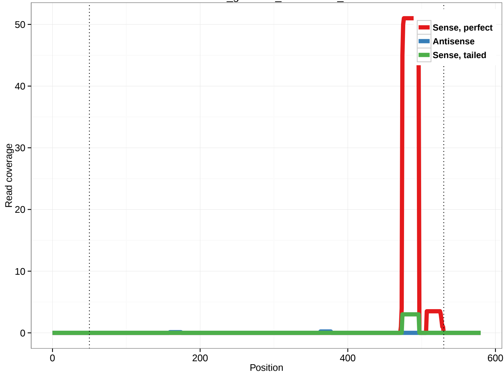
rheMac3_genscan_chr11.1568_9
