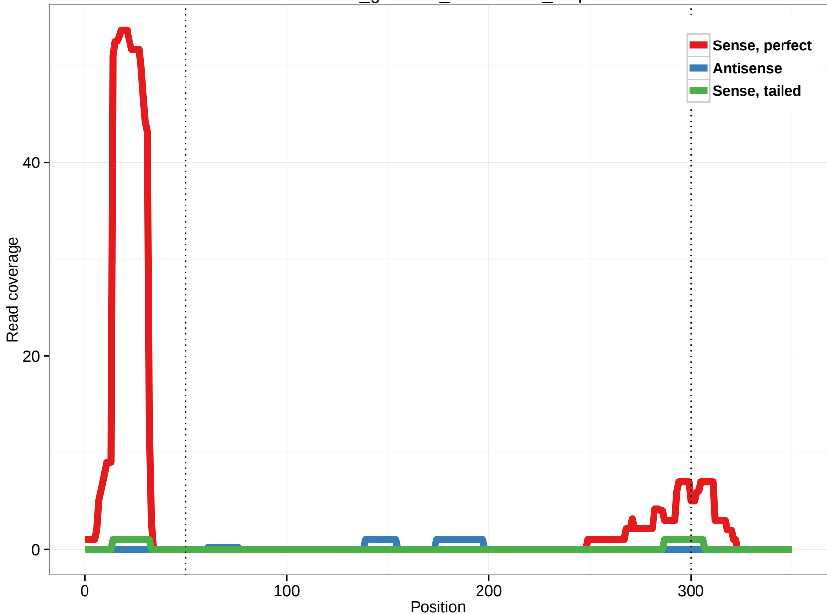
rheMac3_genscan_chr11.1460_0.5p
