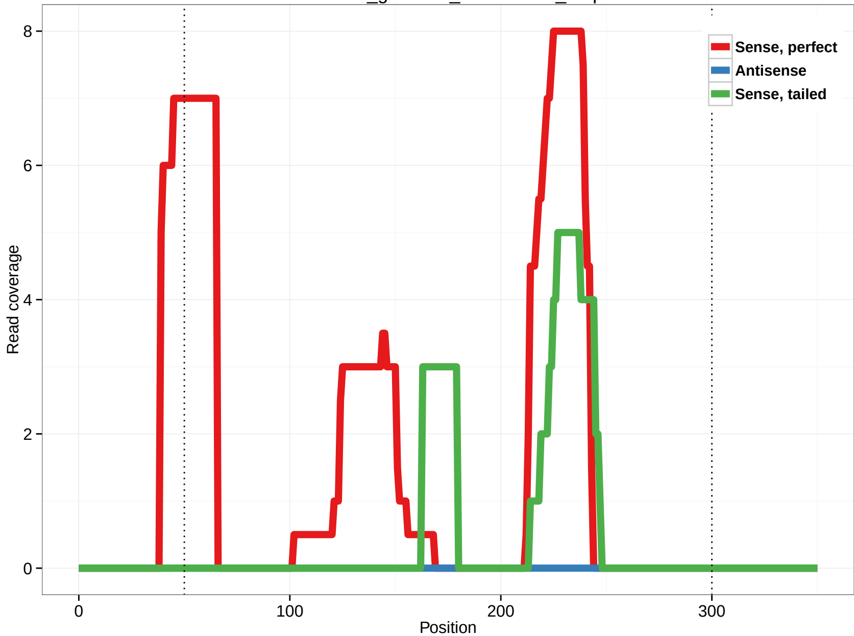
rheMac3_genscan_chr11.1432_4.5p
