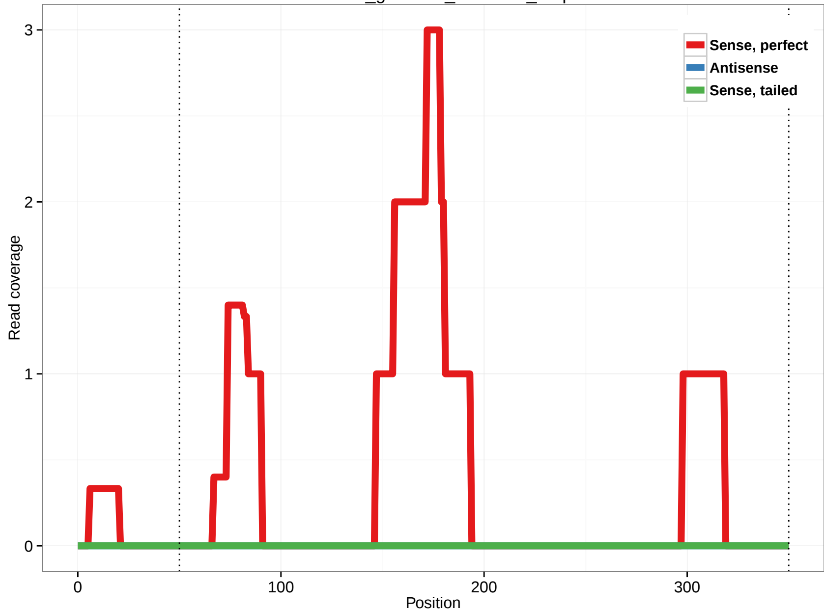
rheMac3_genscan_chr11.13_1.5p
