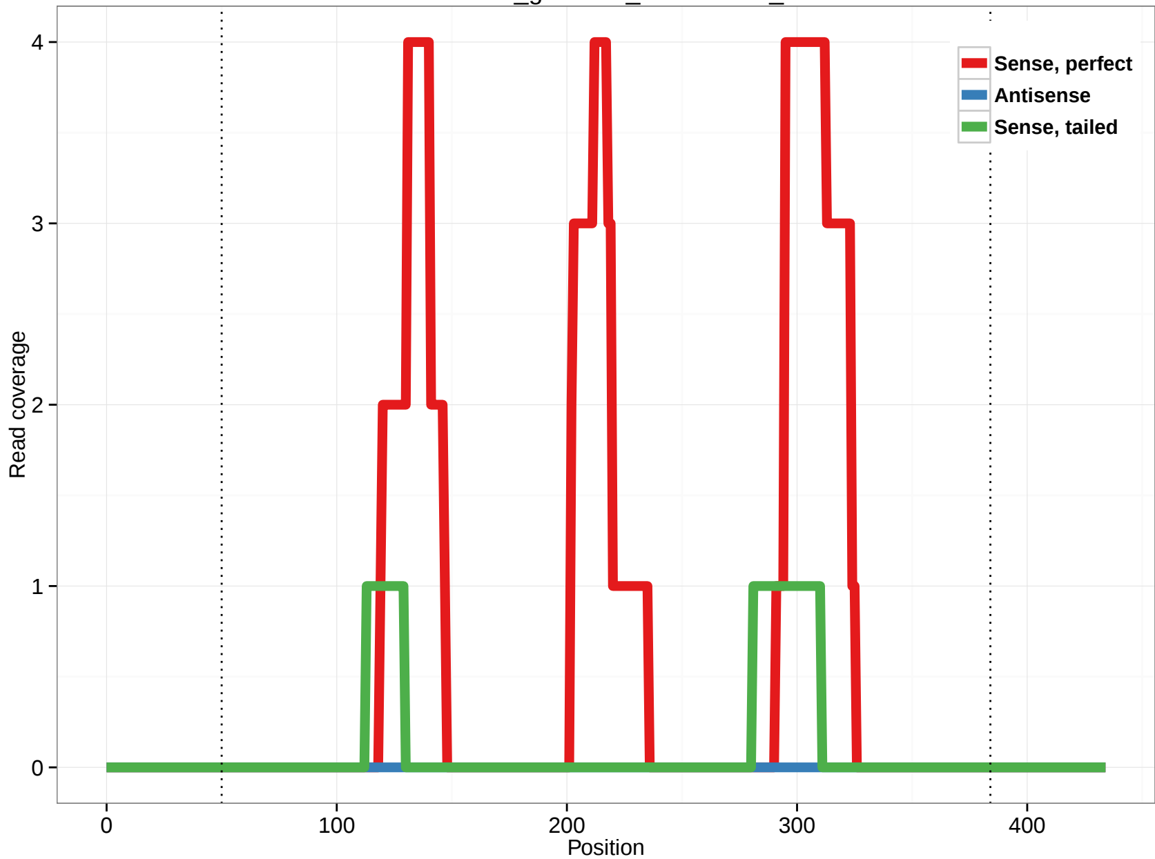
rheMac3_genscan_chr11.1395_1
