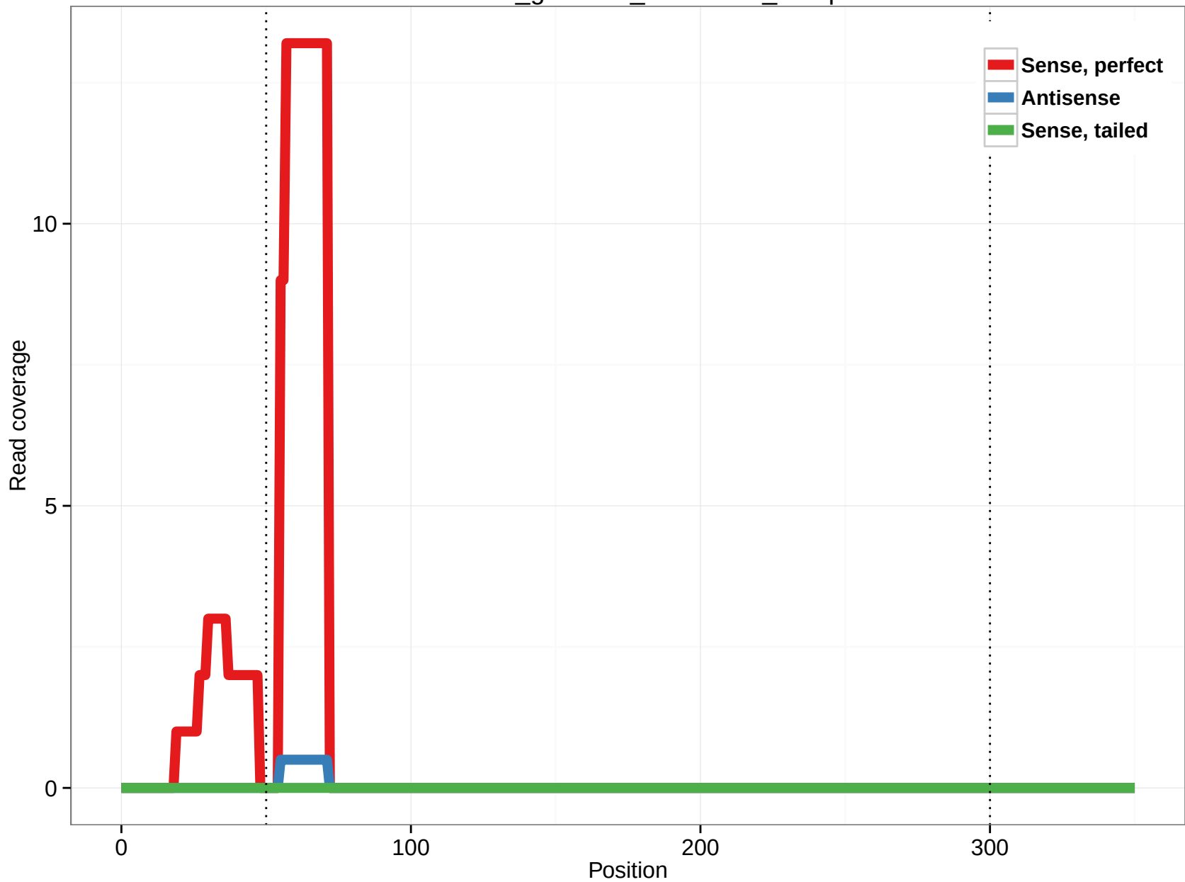
rheMac3_genscan_chr11.134_45.5p
