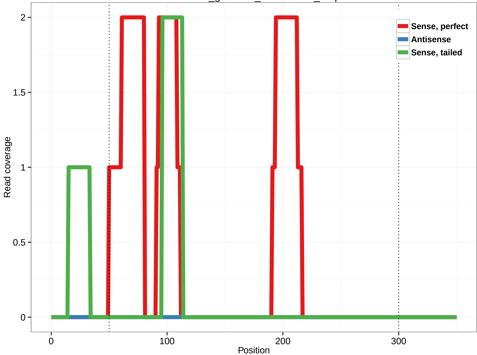
rheMac3_genscan_chr11.1310_6.3p
