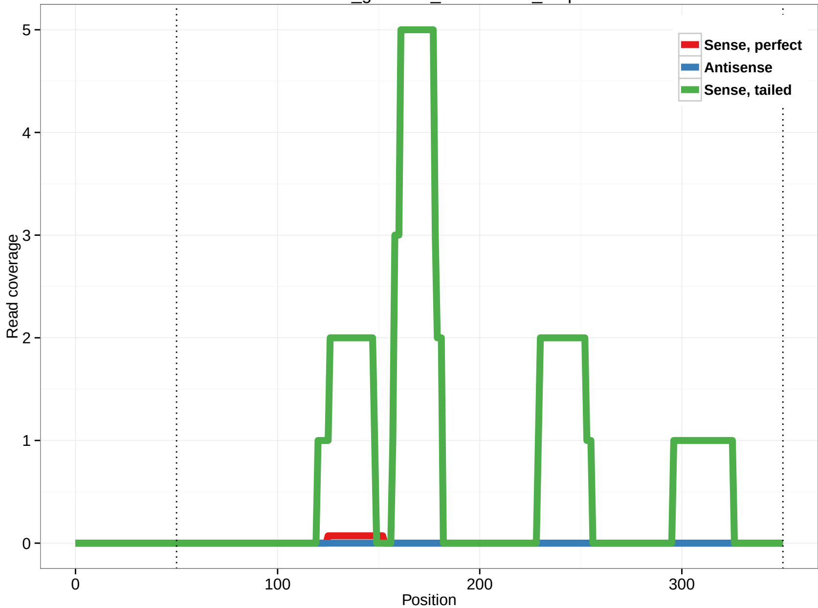
rheMac3_genscan_chr11.1194_0.5p
