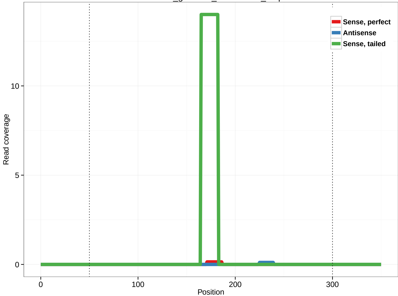
rheMac3_genscan_chr11.1166_3.5p
