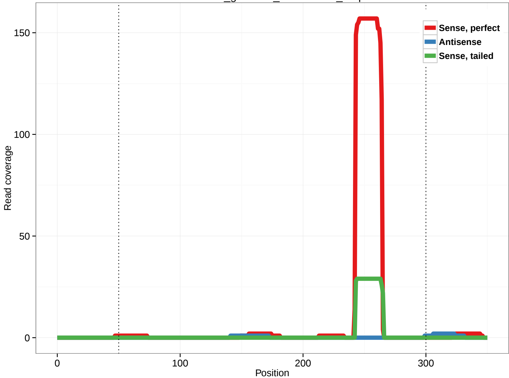
rheMac3_genscan_chr11.1160_9.3p
