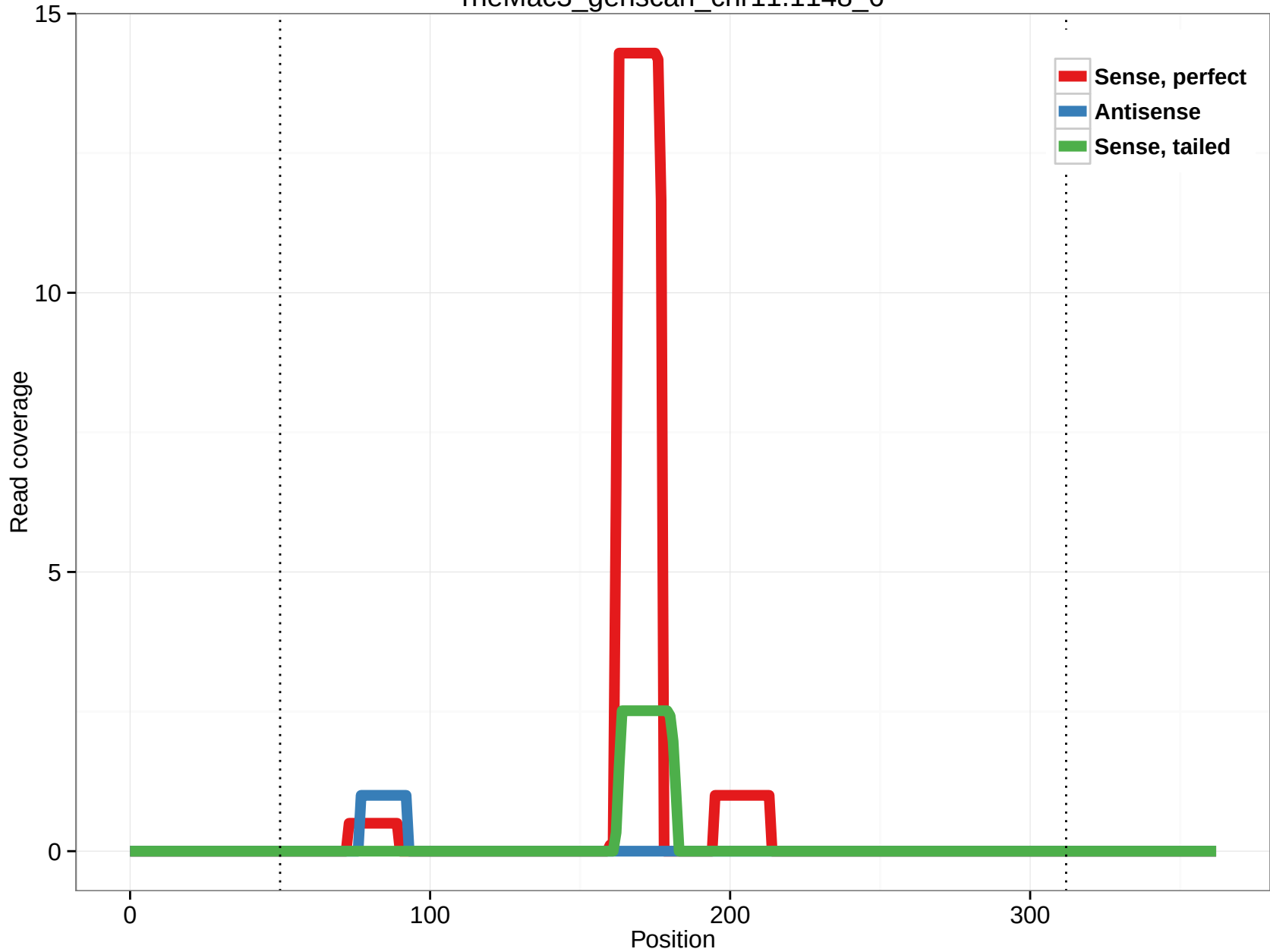
rheMac3_genscan_chr11.1148_6
