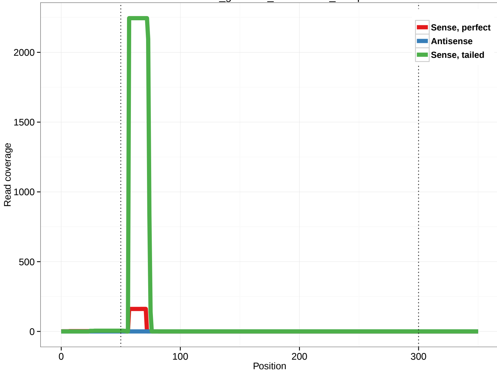
rheMac3_genscan_chr11.1146_13.5p
