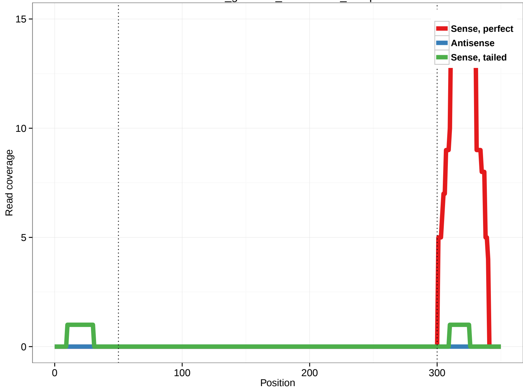
rheMac3_genscan_chr11.1146_13.3p
