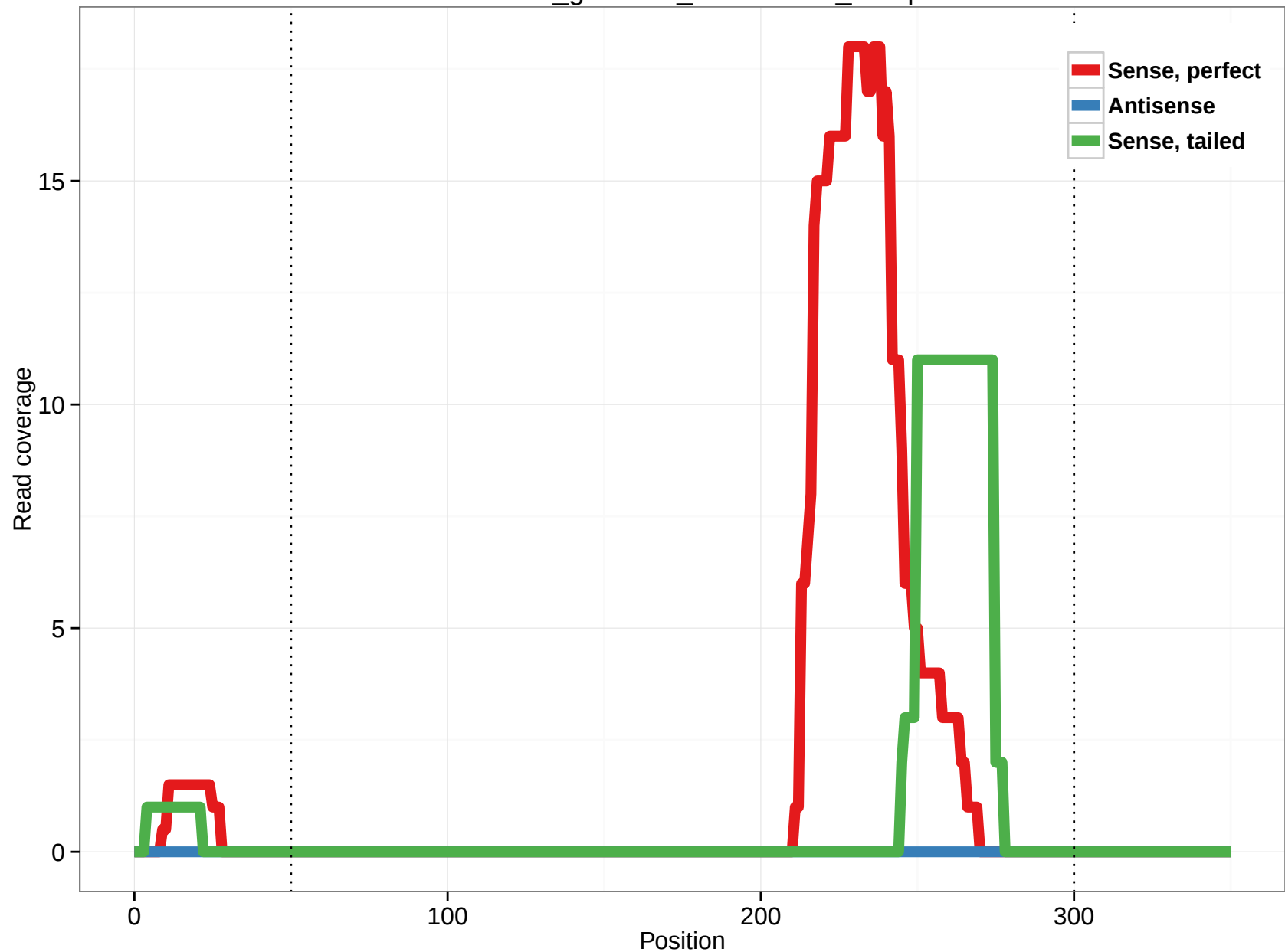
rheMac3_genscan_chr11.1146_10.5p
