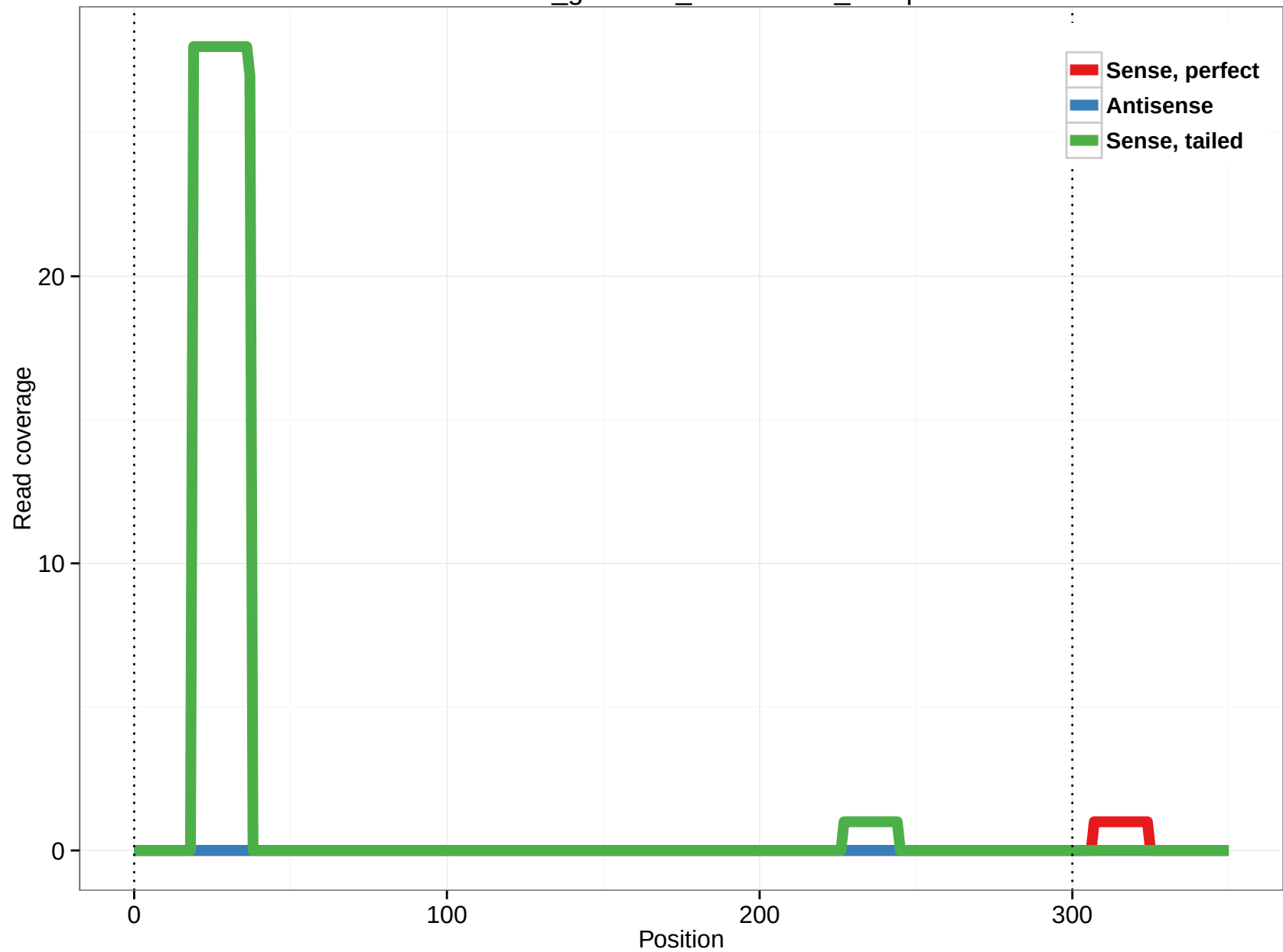
rheMac3_genscan_chr11.1113_16.3p
