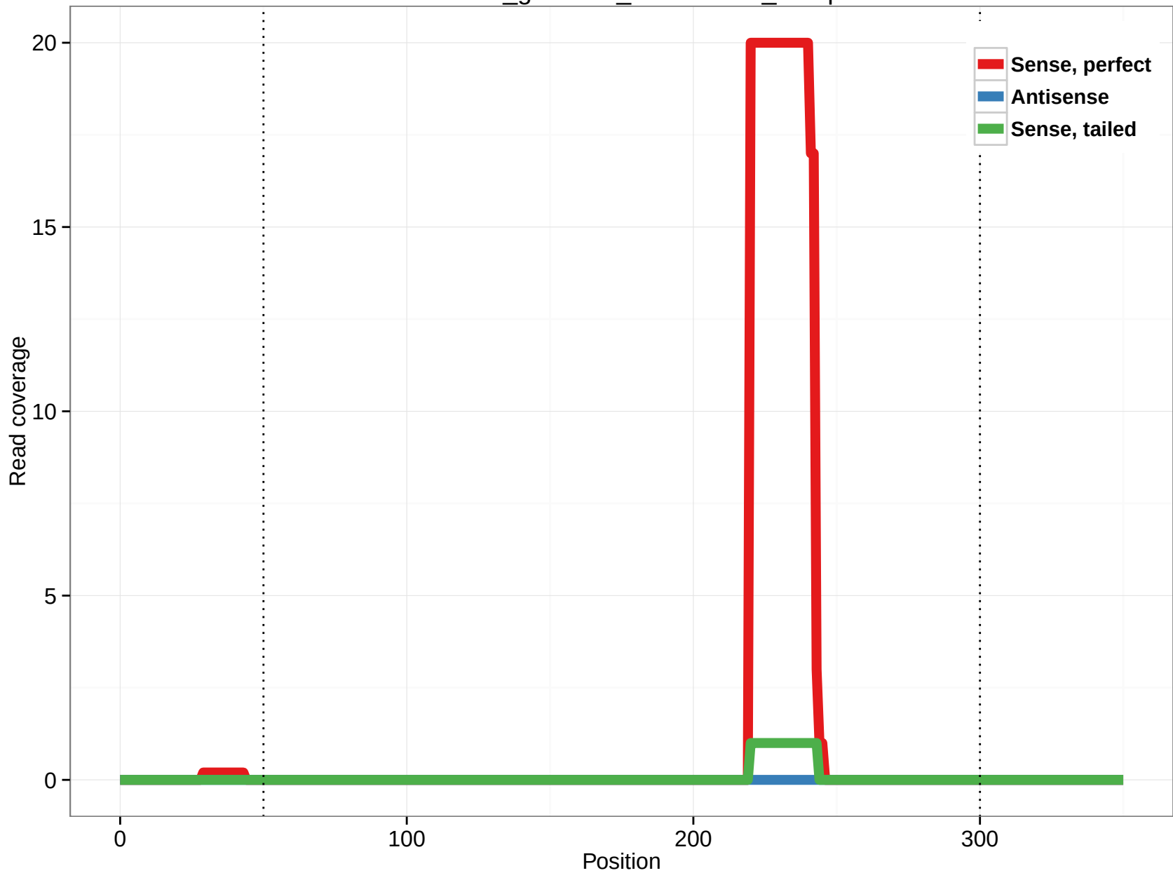
rheMac3_genscan_chr11.1110_41.5p
