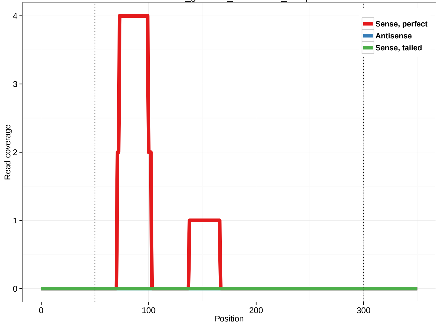
rheMac3_genscan_chr11.1099_34.5p
