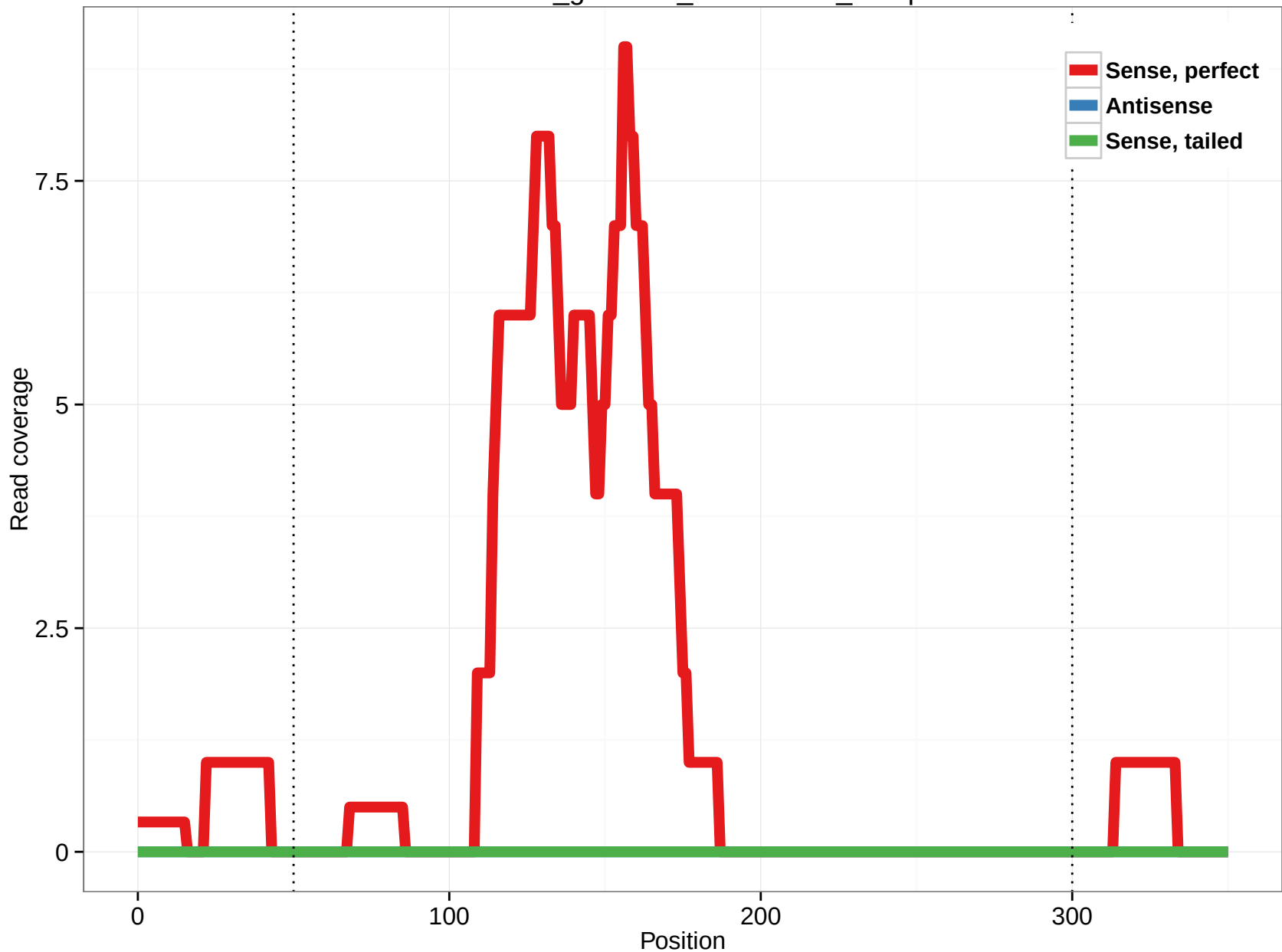
rheMac3_genscan_chr11.1099_31.5p
