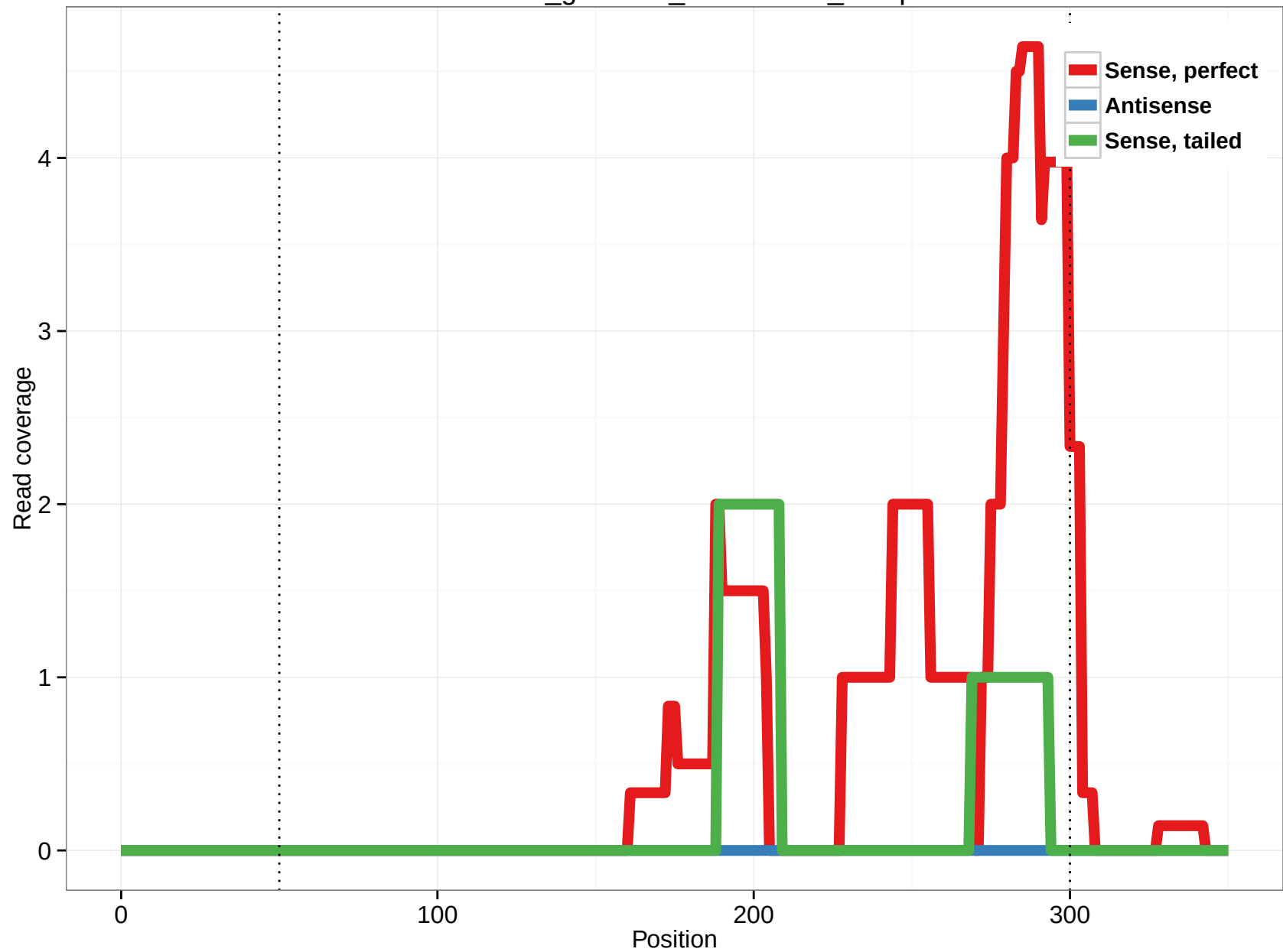
rheMac3_genscan_chr11.1099_29.3p
