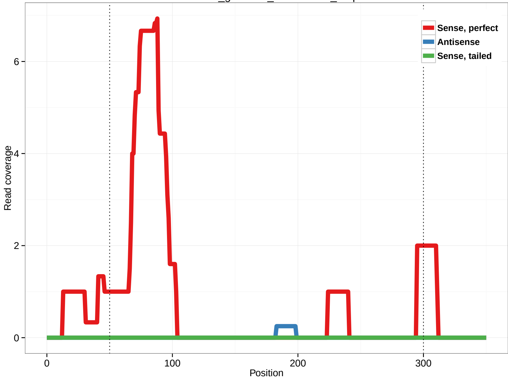
rheMac3_genscan_chr11.1083_4.3p
