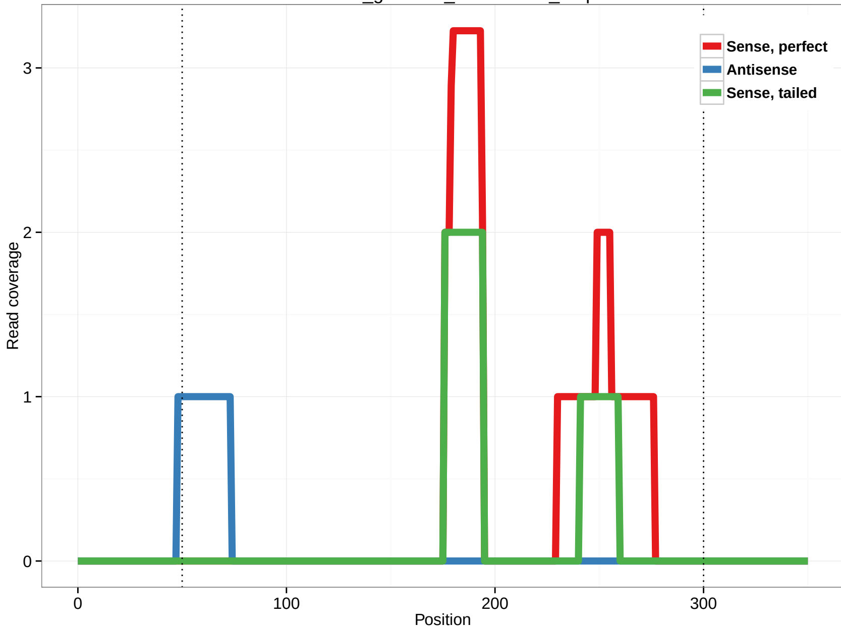
rheMac3_genscan_chr11.1079_0.3p
