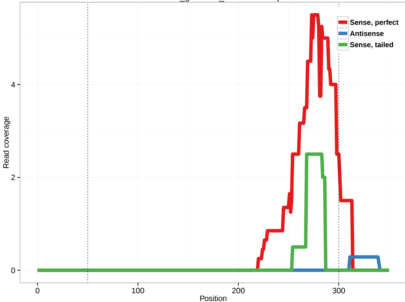
rheMac3_genscan_chr11.1033.3p
