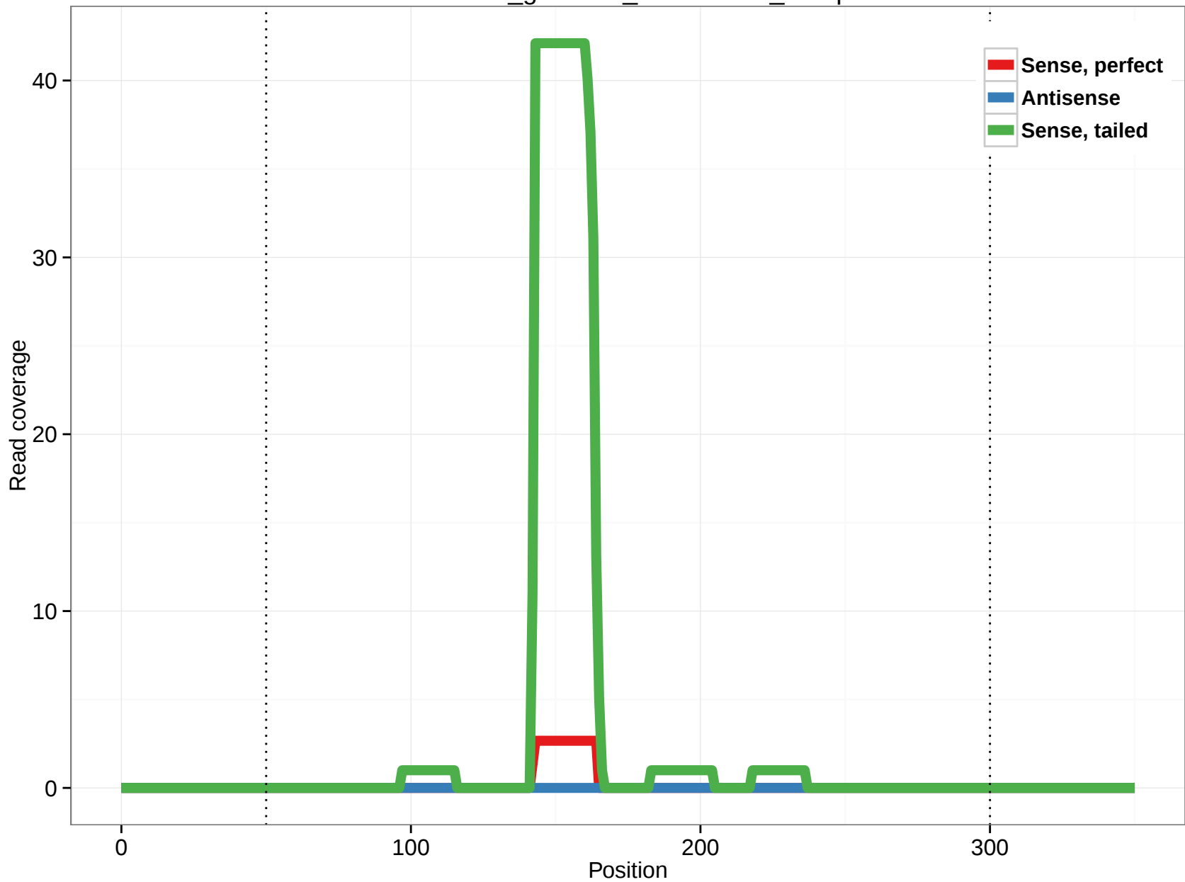
rheMac3_genscan_chr11.1016_20.5p
