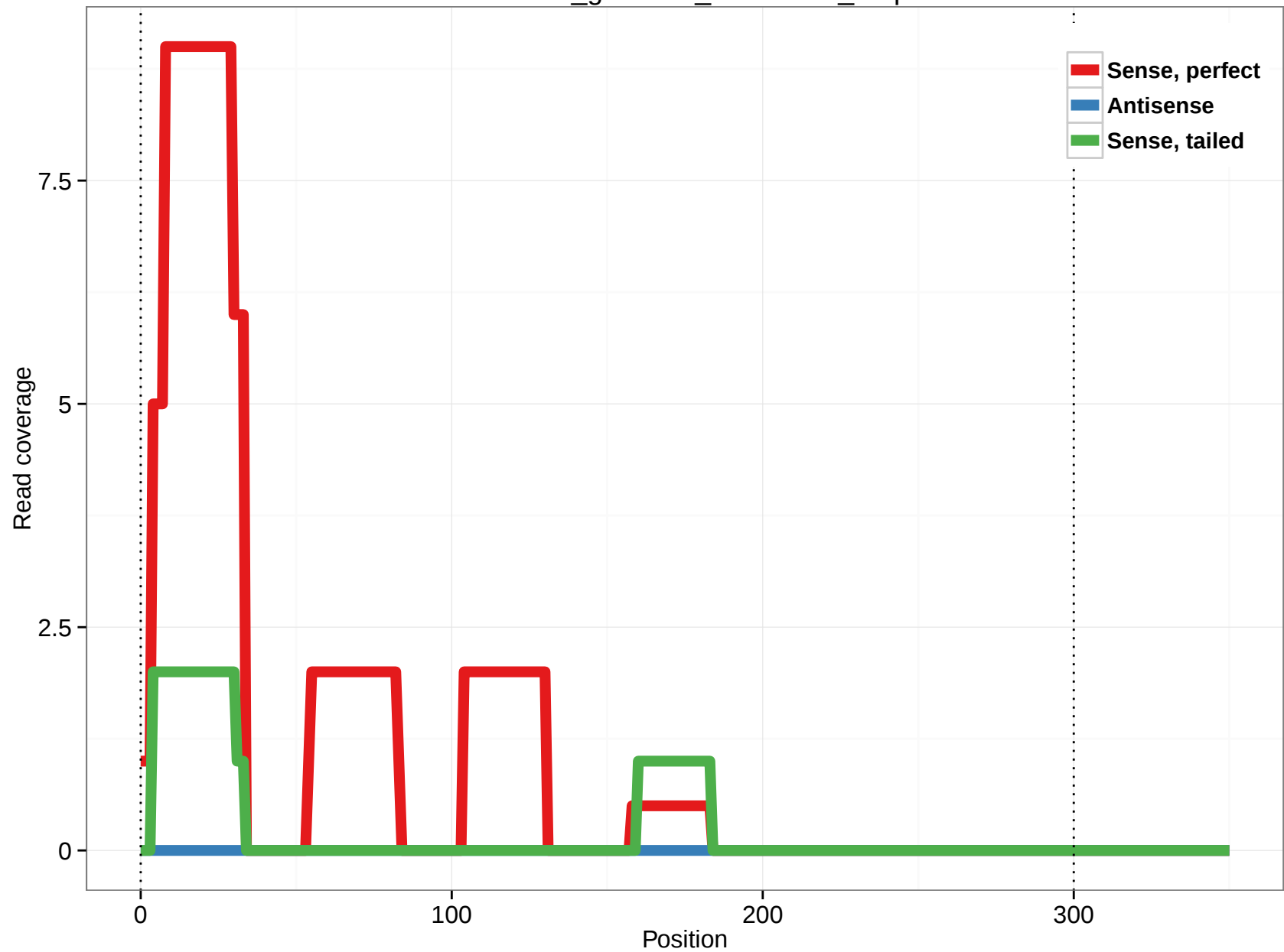
rheMac3_genscan_chr10.977_6.3p
