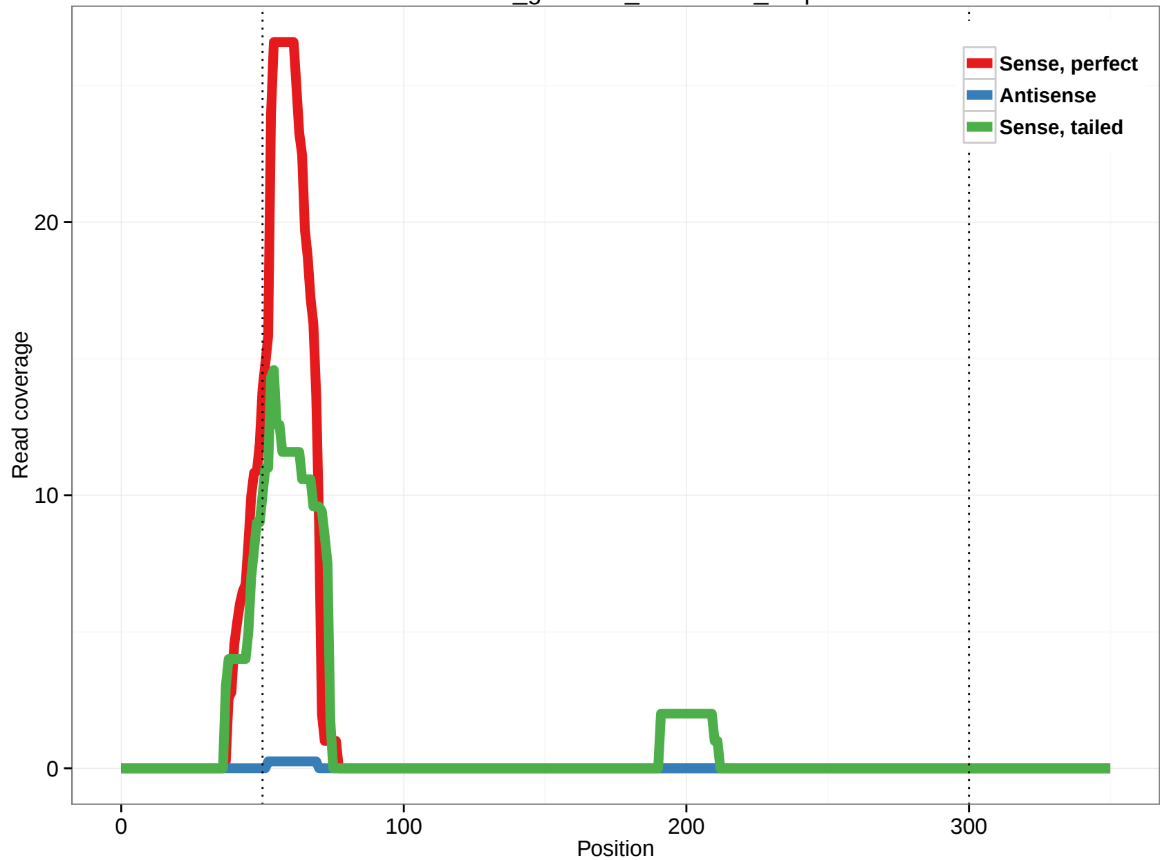
rheMac3_genscan_chr10.922_2.3p
