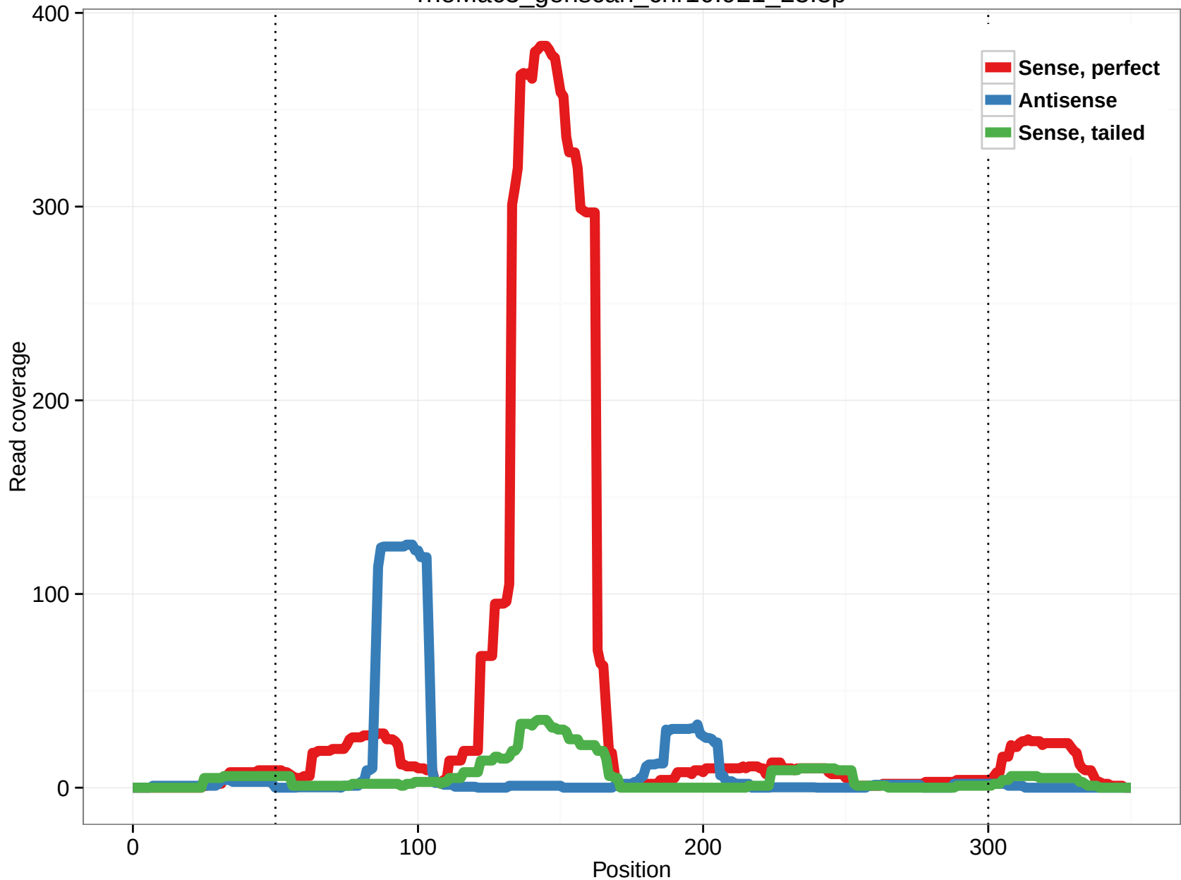
rheMac3_genscan_chr10.921_23.3p
