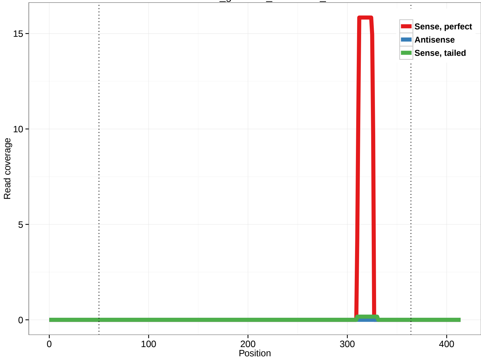
rheMac3_genscan_chr10.911_4
