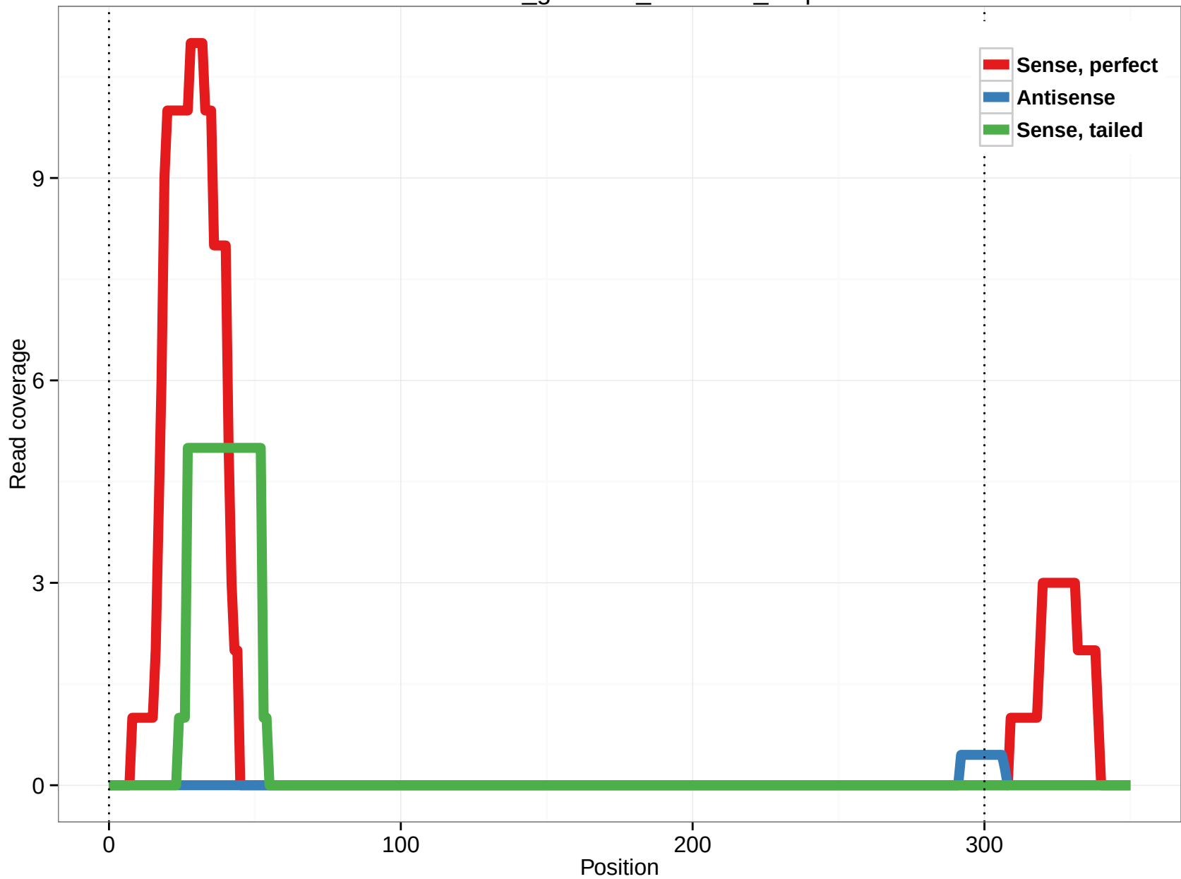
rheMac3_genscan_chr10.89_4.3p
