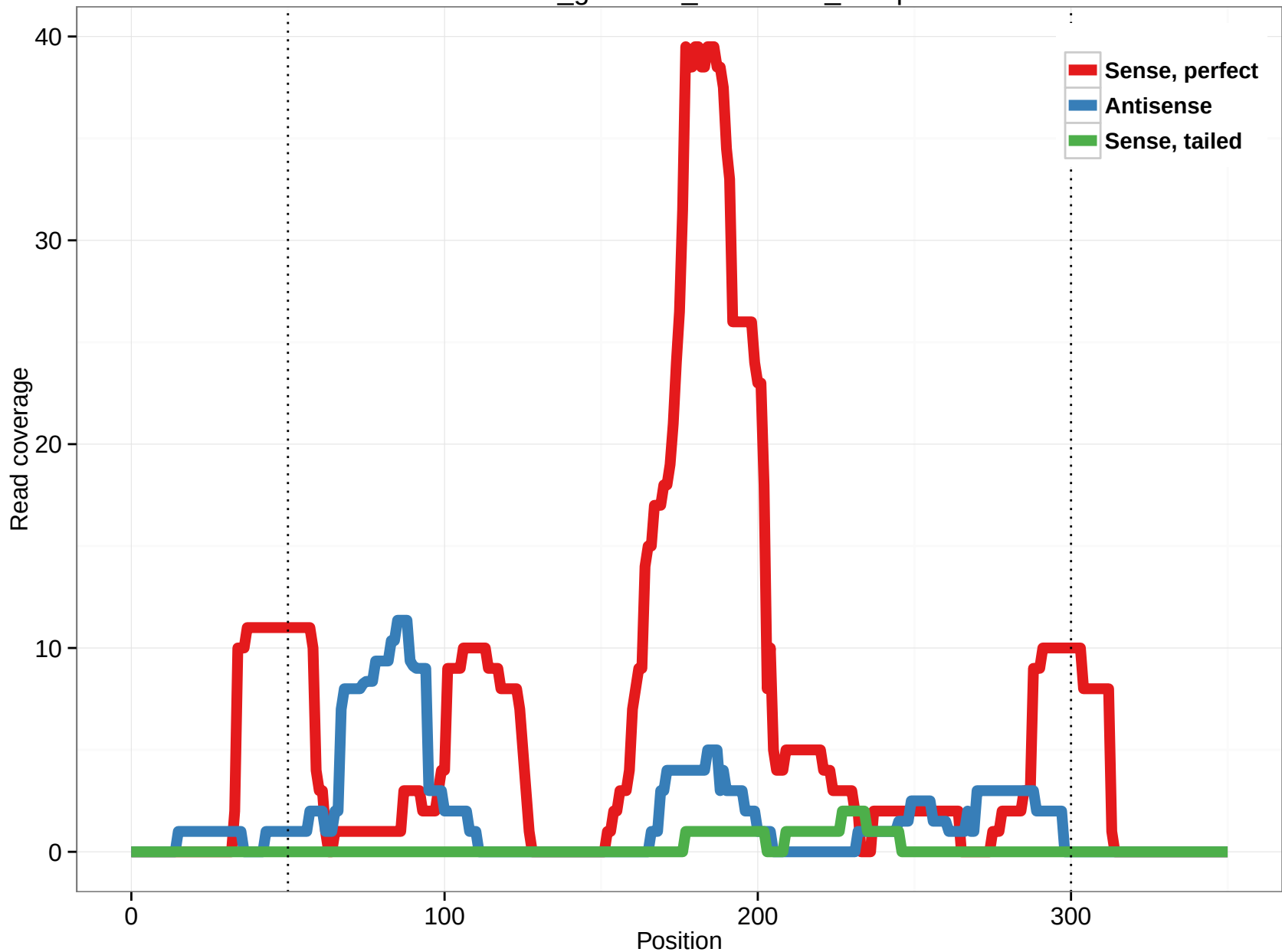
rheMac3_genscan_chr10.883_10.5p
