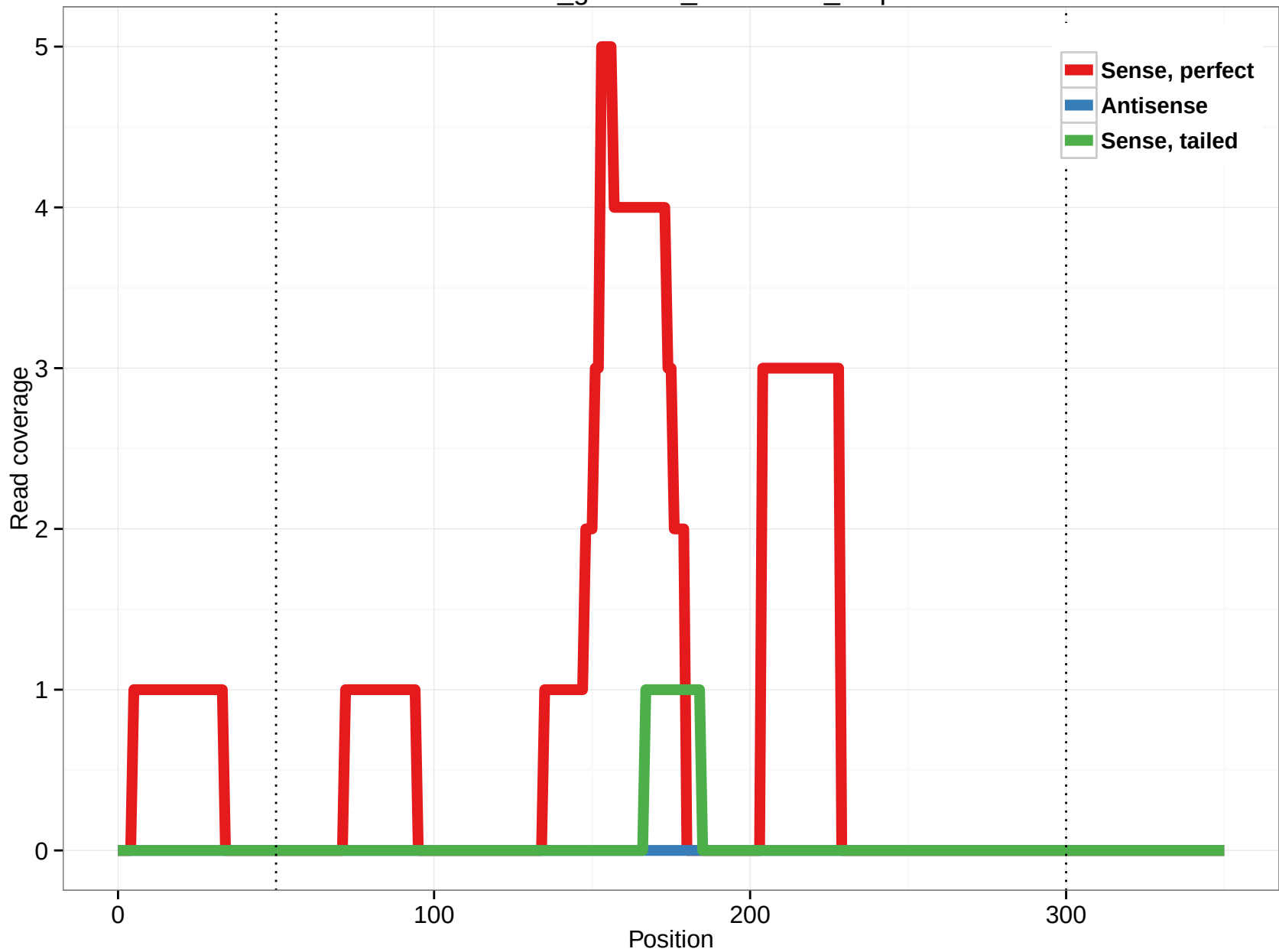
rheMac3_genscan_chr10.873_0.5p
