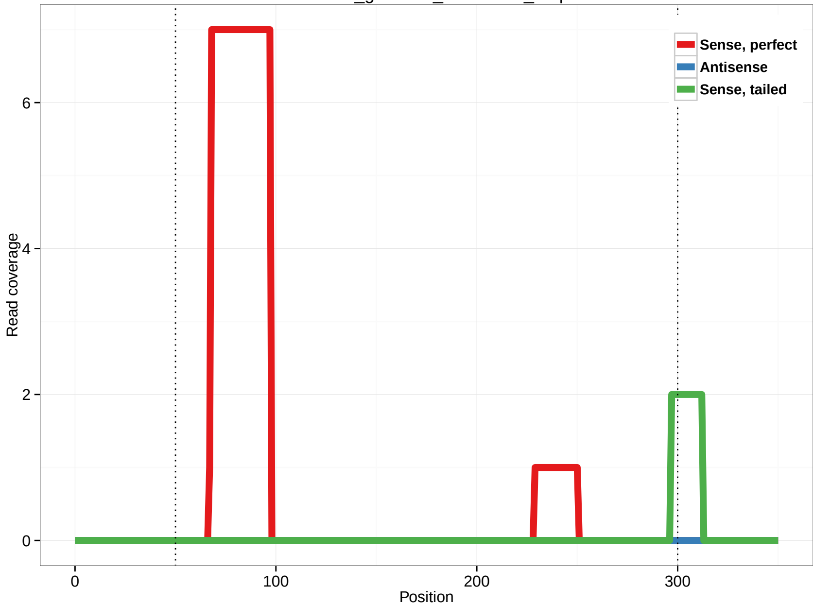
rheMac3_genscan_chr10.806_9.3p
