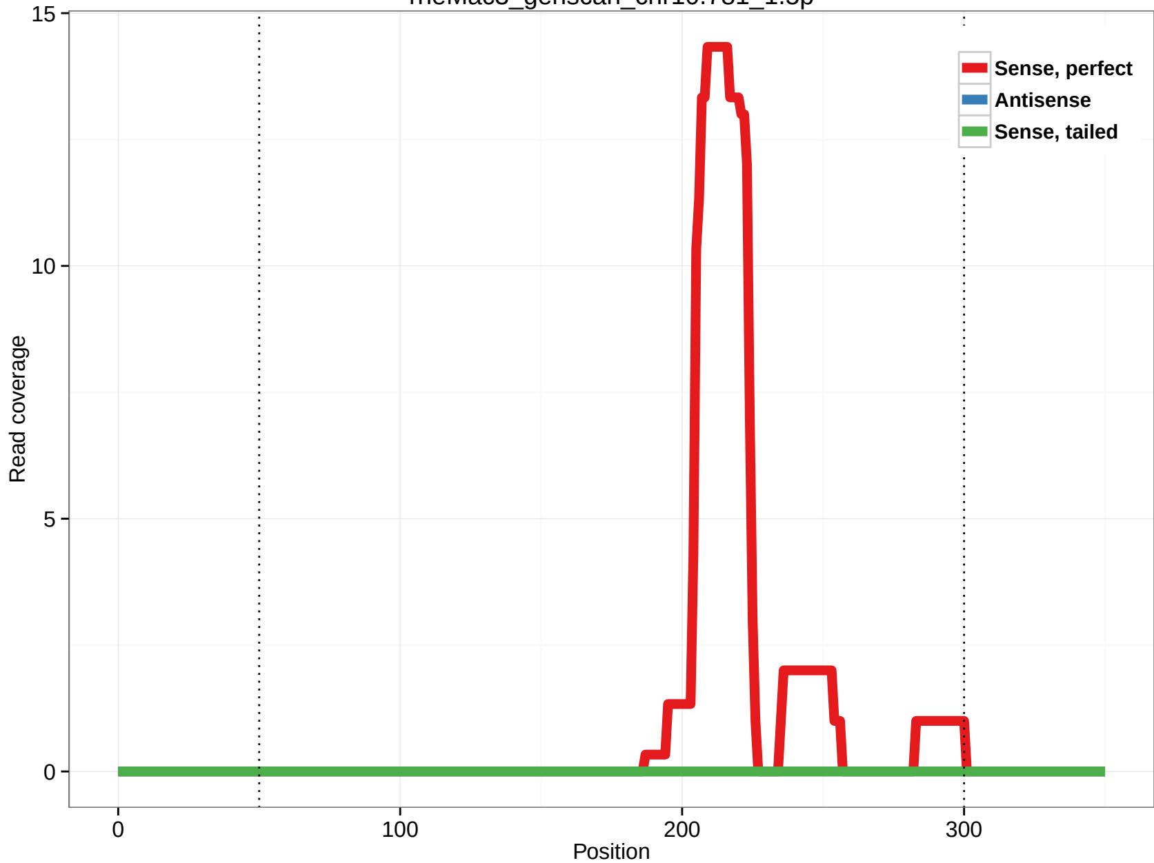
rheMac3_genscan_chr10.781_1.5p
