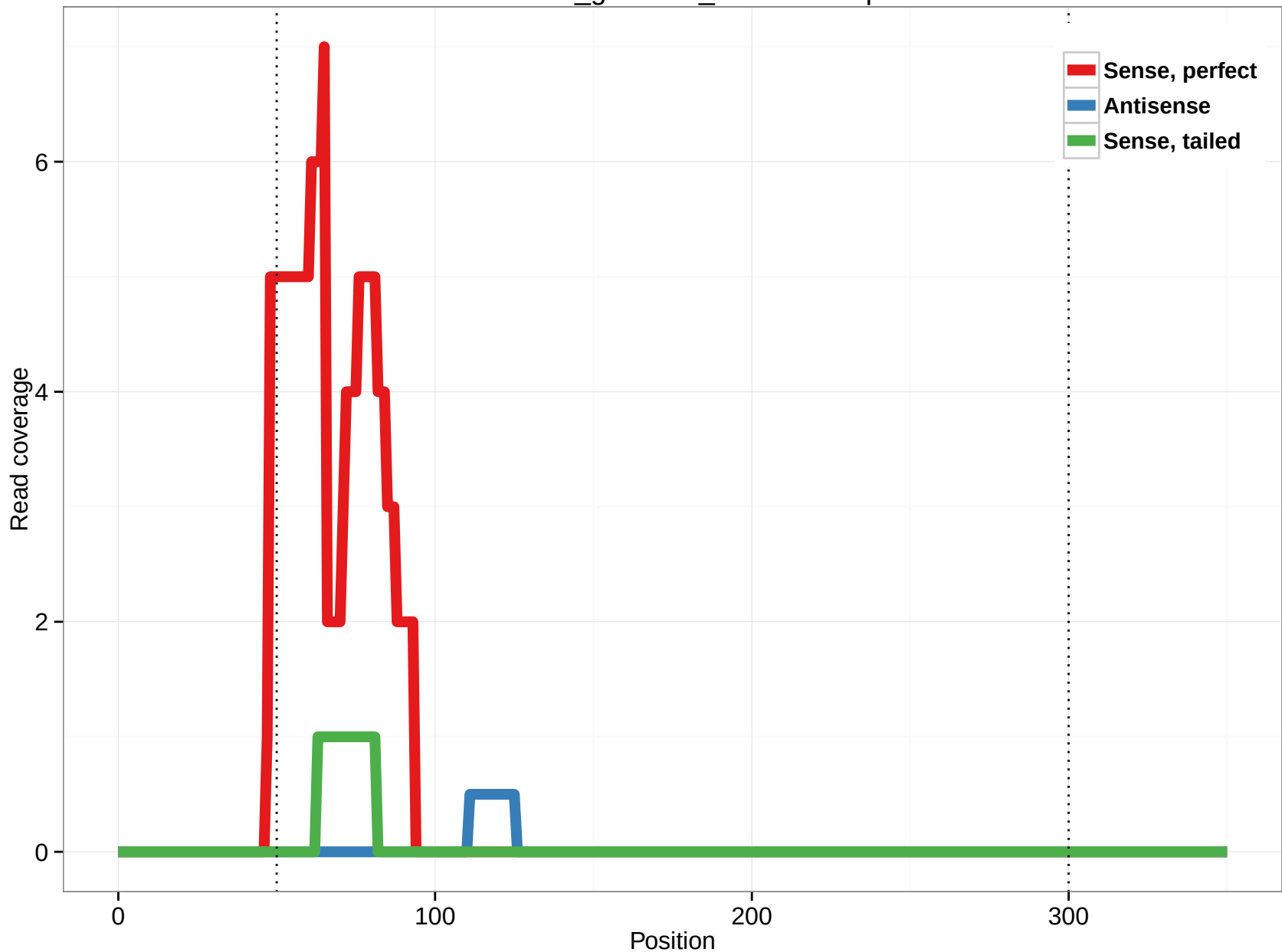
rheMac3_genscan_chr10.780.5p
