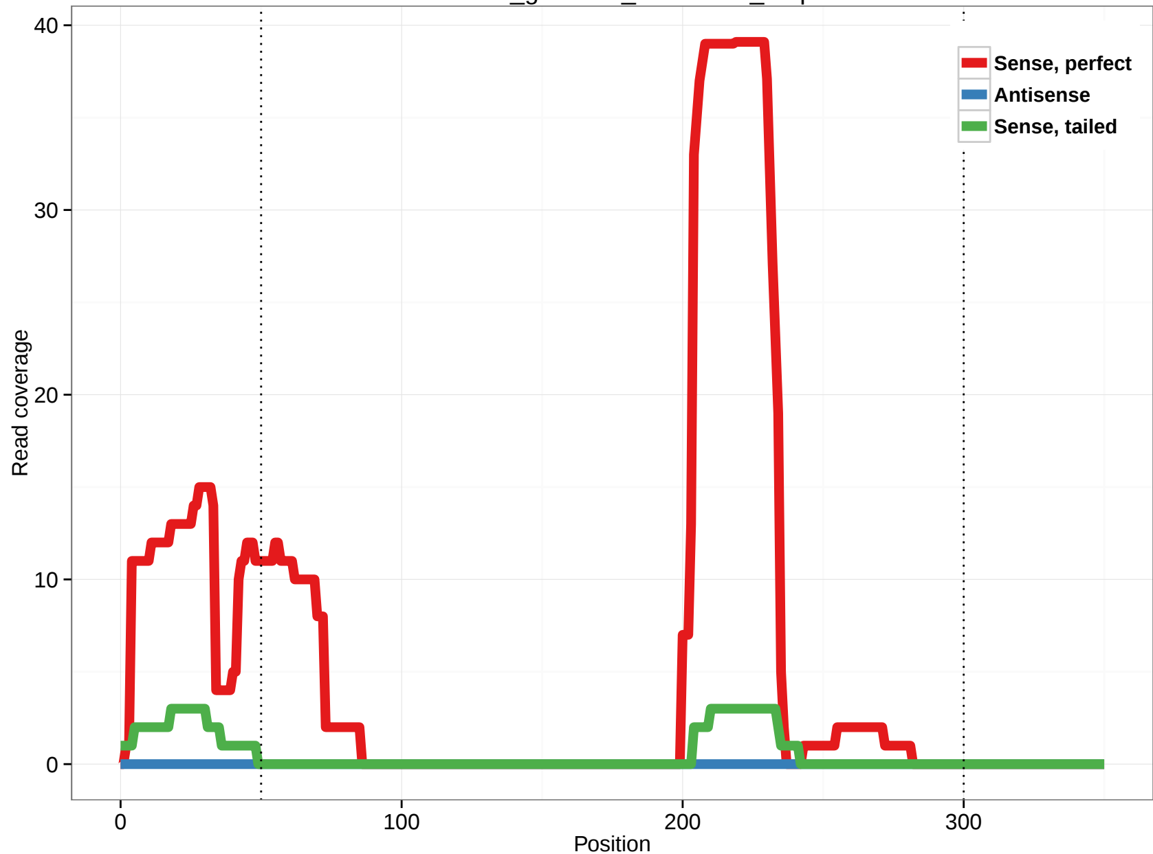
rheMac3_genscan_chr10.740_6.5p
