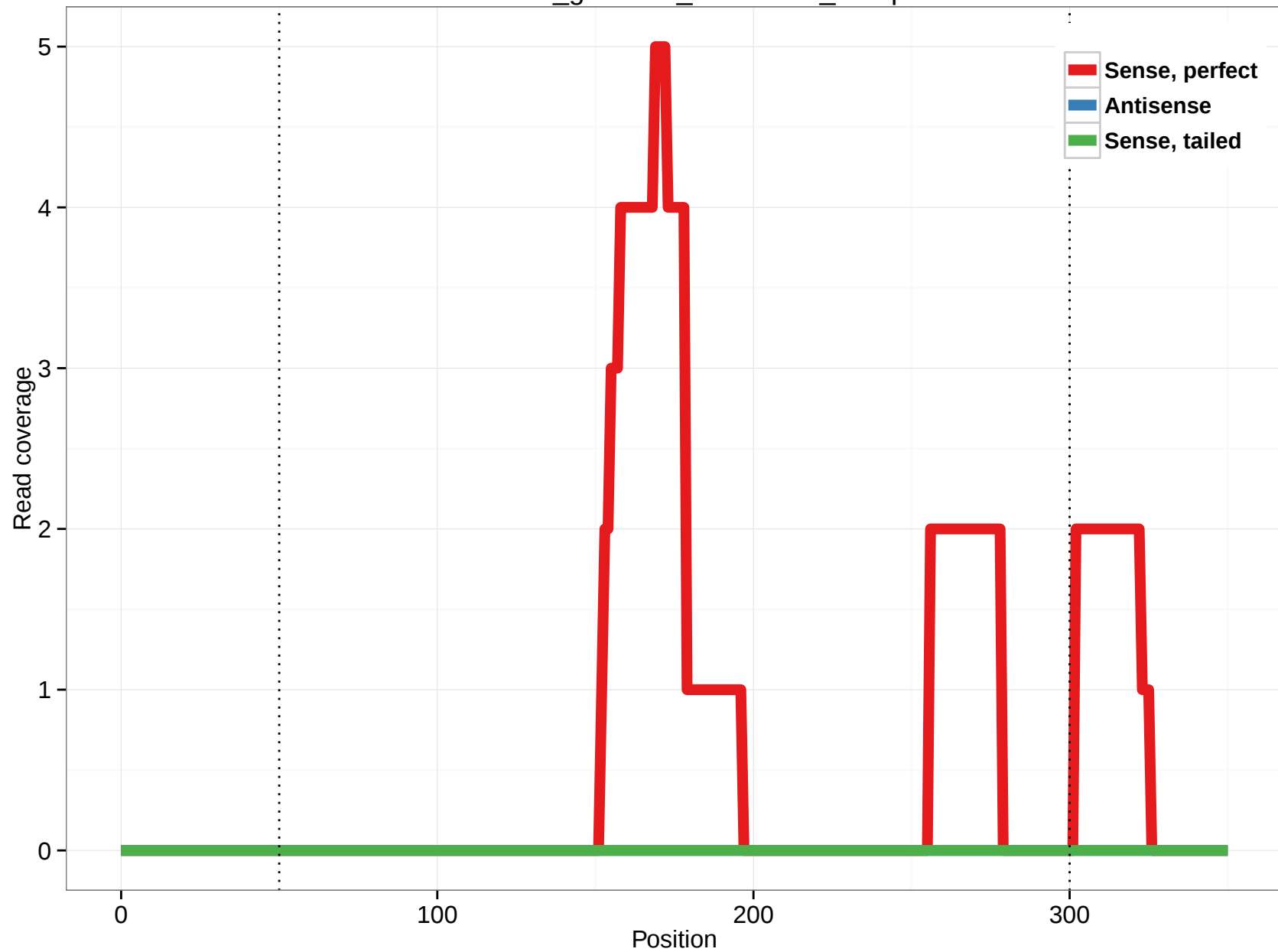
rheMac3_genscan_chr10.633_14.3p
