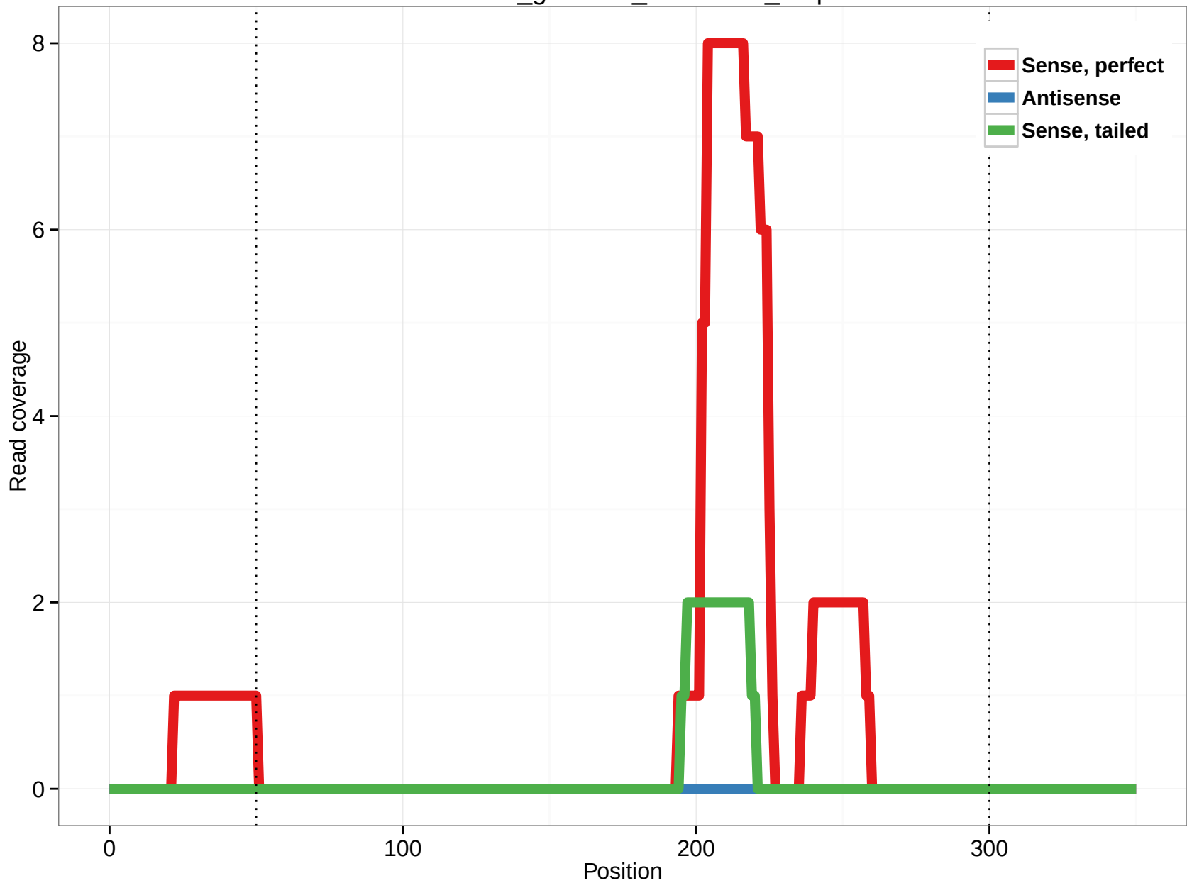
rheMac3_genscan_chr10.629_2.3p
