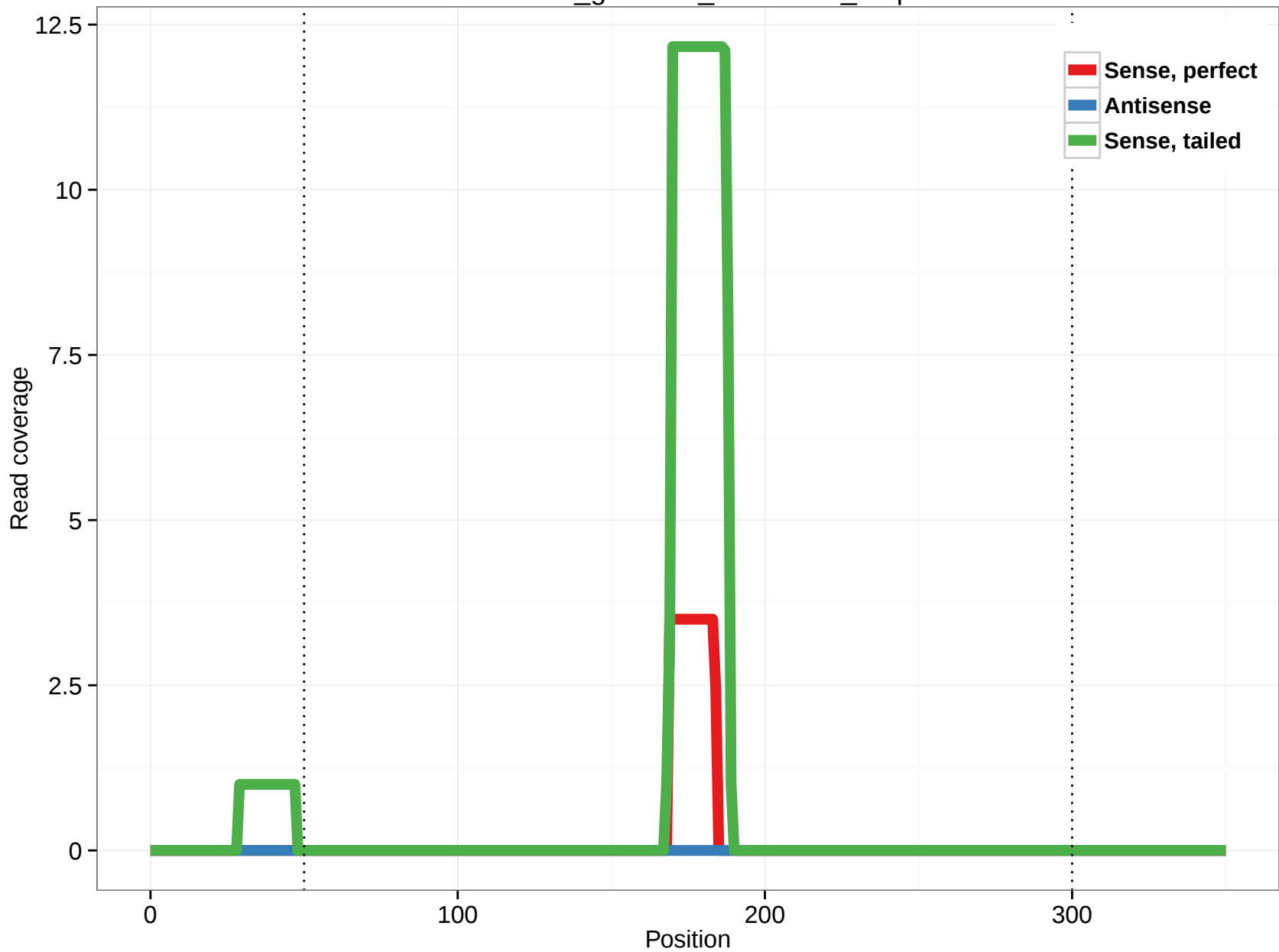
rheMac3_genscan_chr10.625_0.3p
