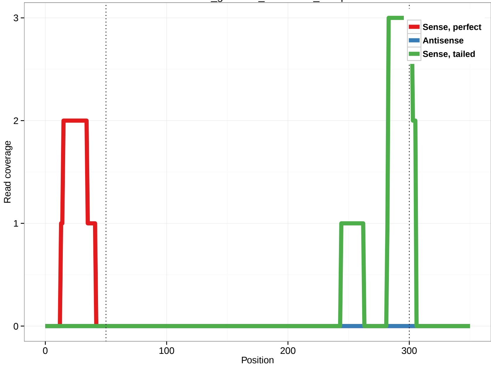
rheMac3_genscan_chr10.617_27.5p
