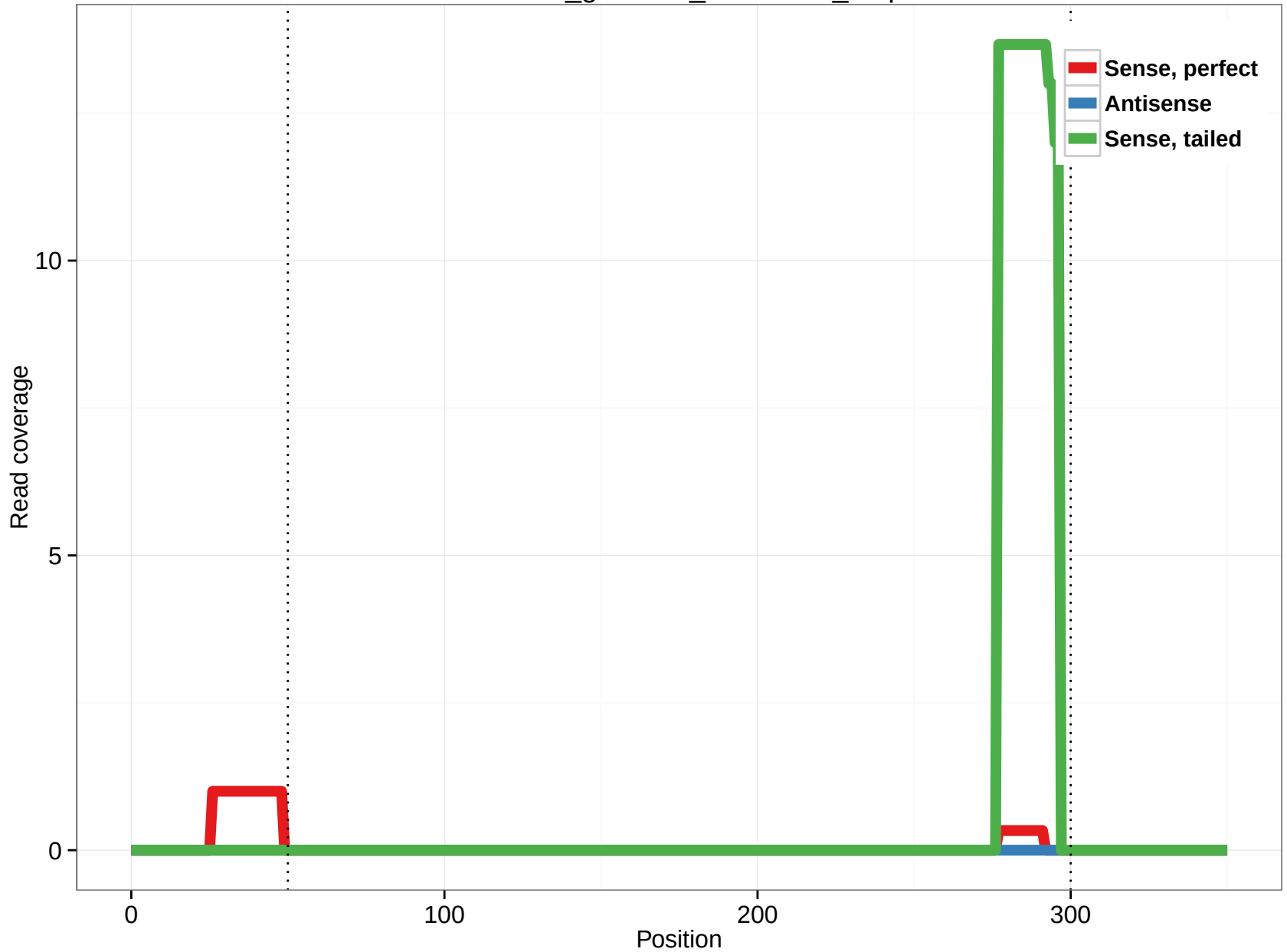
rheMac3_genscan_chr10.604_5.5p
